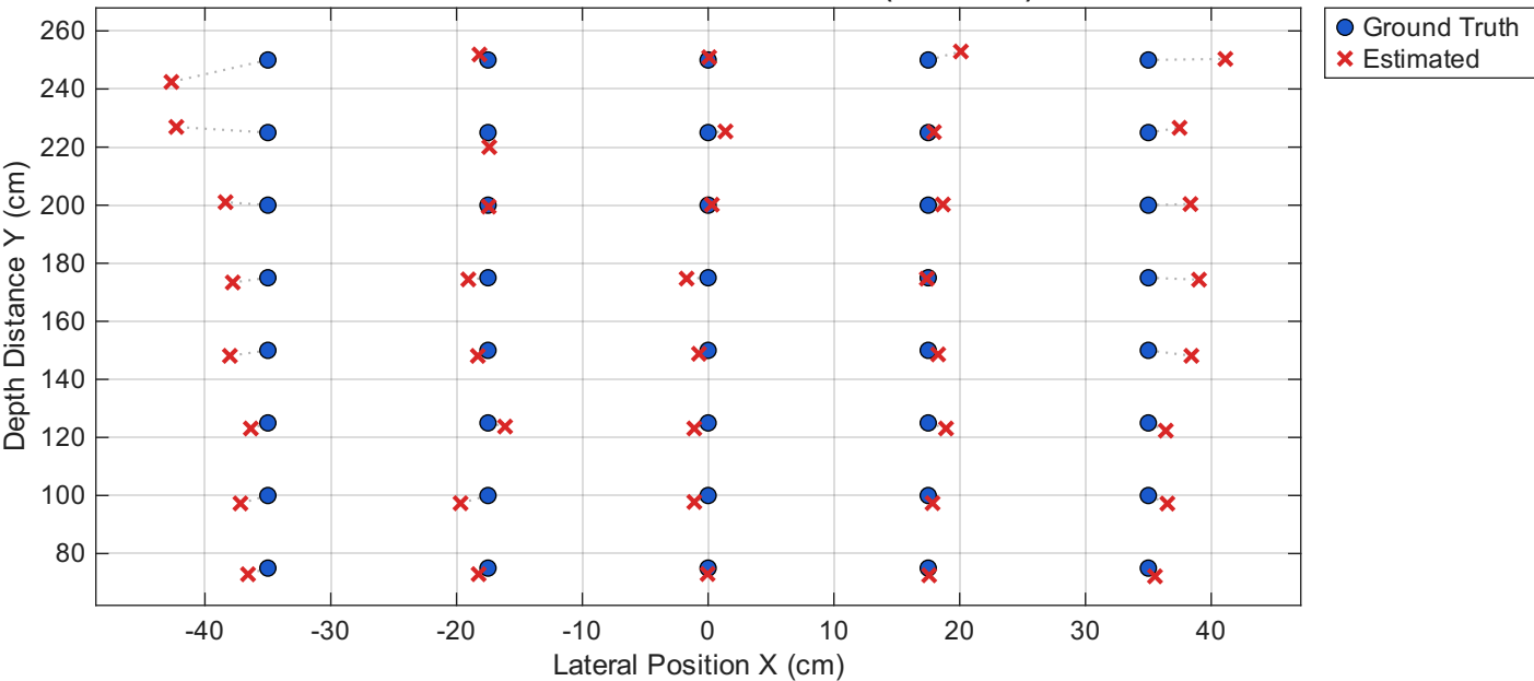
Ground Truth vs. Estimated Positions (X-Y Plane)
