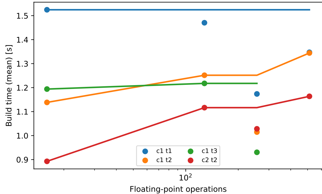
Build time scaling
