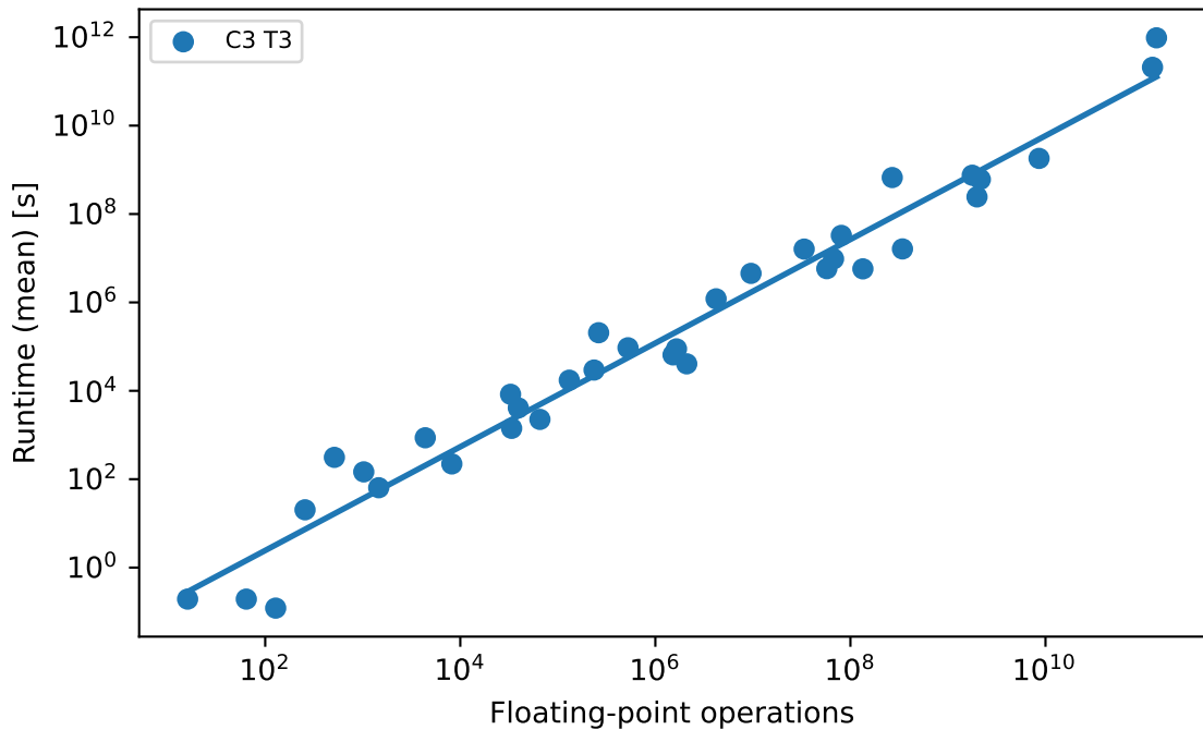
Scaling comparison
