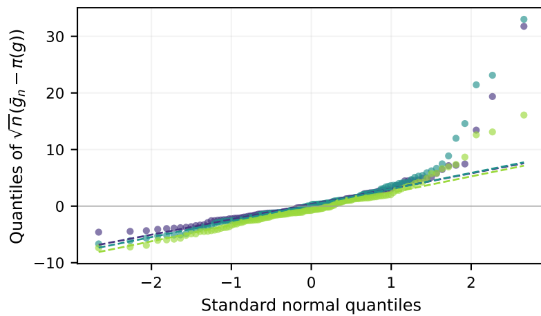
MH-HMC, L=10
