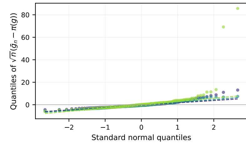
MH-HMC, L=5
