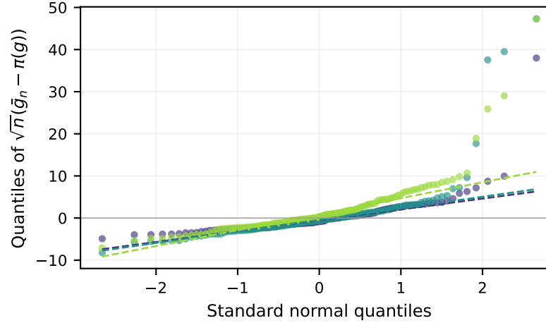
MH-HMC, L~Unif[1,10]
