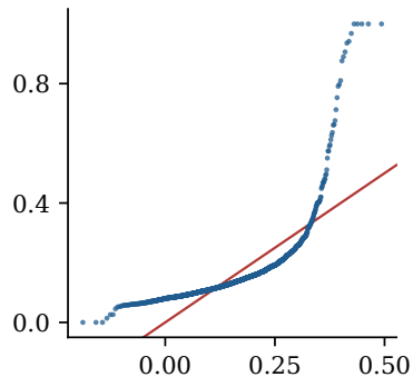
(a) ULA T = 1
