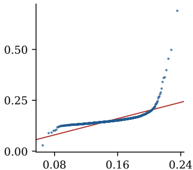
(b) Unadjusted HMC T = 10
