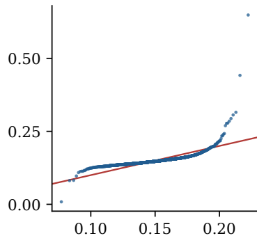
(c) Unadjusted HMC T \sim \text{Unif}\{1, \dots, 19\}
