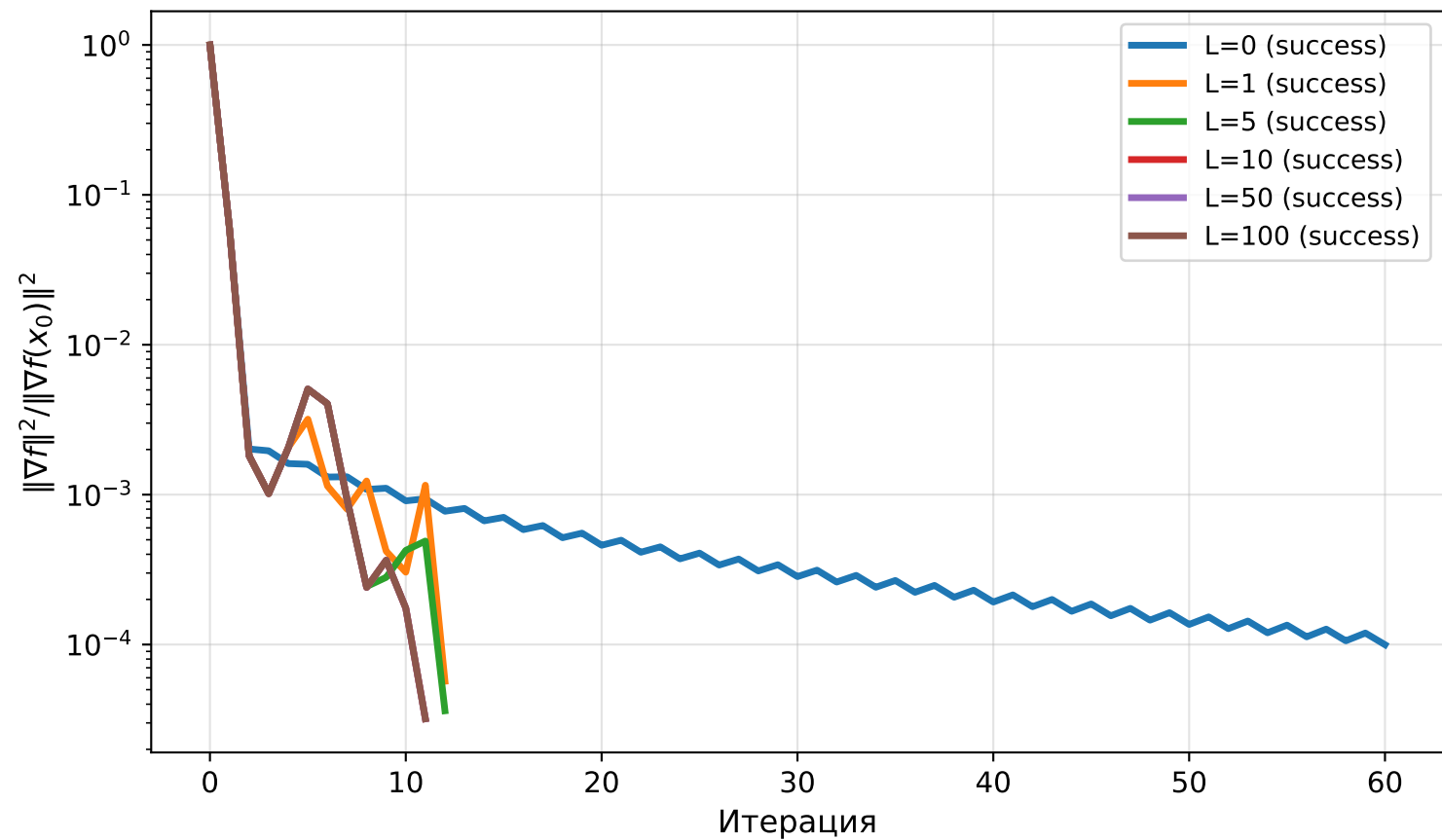
П. 2.3 (a): triazines (Pseudo-Huber), L-BFGS
