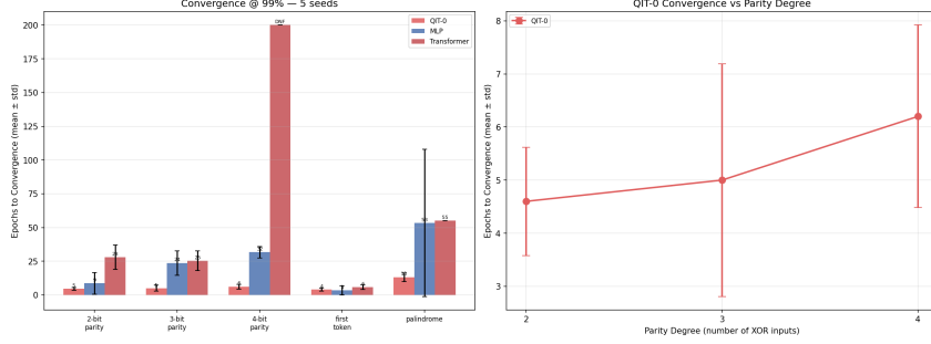
Figure 5: Task variety benchmark (5 seeds). Left : convergence epoch by task and model (DNF shown at epoch limit). Right : QIT-0 parity-degree scaling — a monotonic, graceful increase from 4.6 \pm 1.0 (2-bit) to 6.2 \pm 1.7 (4-bit).
