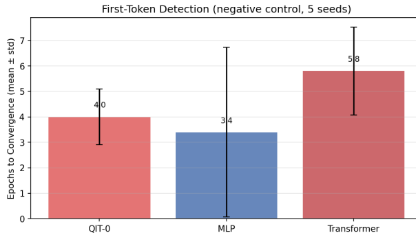
Figure 4: First-token detection (negative control): convergence epoch comparison (5 seeds each). QIT-0 is not faster than classical models on this positional task with no quantum phase structure.
