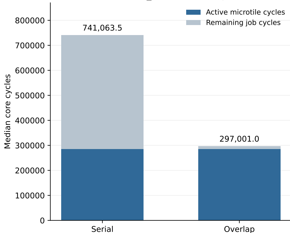
Recorded JOB_CYCLES decomposition
