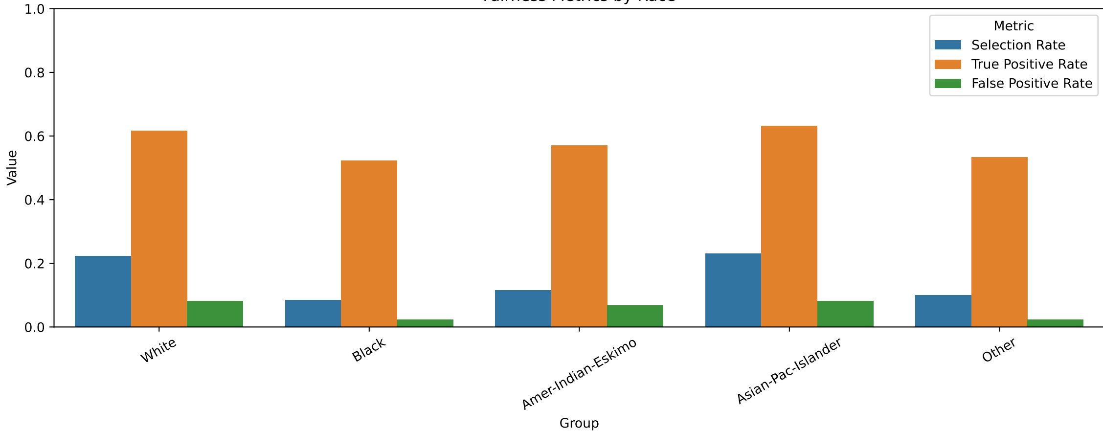
Fairness Metrics by Race
