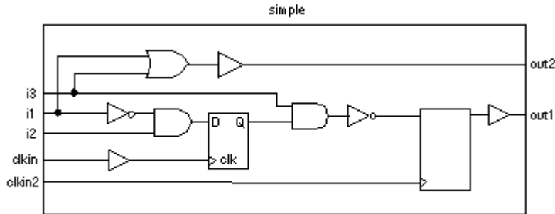
Figure 4-2 Gate-Level Netlist
