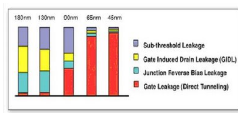
Figure 4. Technology shrinking vs. Leakage components
