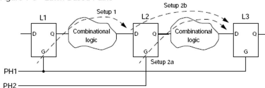
Figure 1-8 Latch-Based Paths
