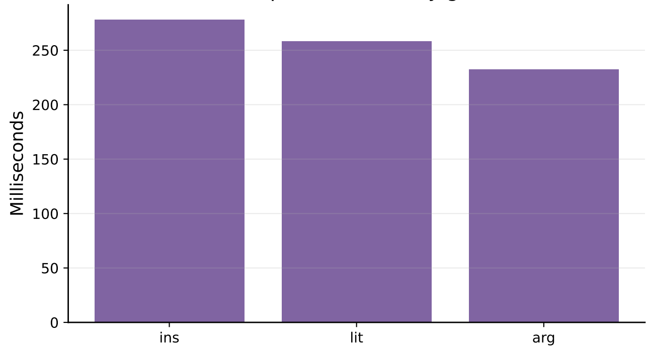
Mean predicted TRT by genre
