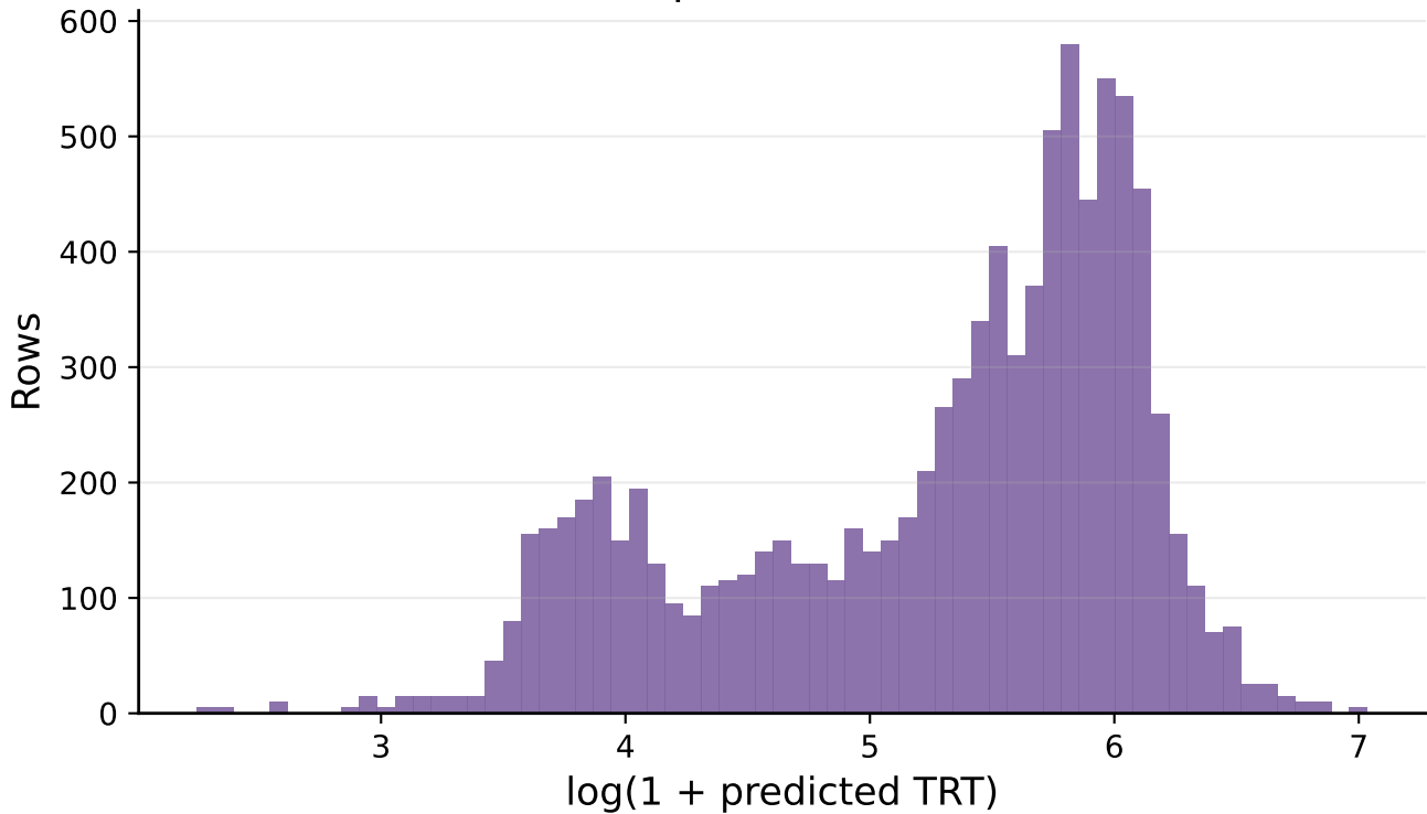
Submission prediction distribution
