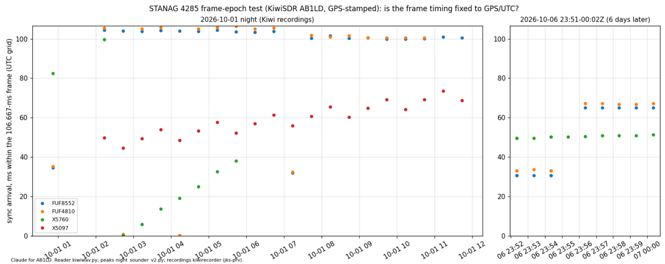
Fig. 4. Sync arrival time within the frame, against the UTC grid, for four STANAG 4285 transmissions. Left: 2026-10-01 night. Right: 2026-10-06, six days later.
