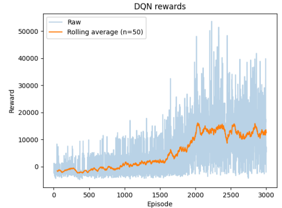
Figure 5: Offensive Agent v.s. Agent Opponent v1 (OFAG1).
