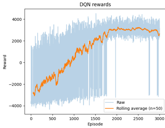
Figure 12: Defensive Agent v.s. Random Opponent v2 (DFRA2).
