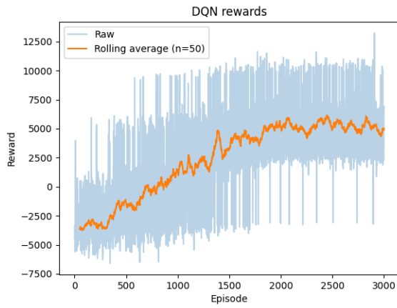
Figure 11: Defensive Agent v.s. Random Opponent v1 (DFRA1).
