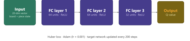
Figure 2: Network architecture of the DQN agent.
