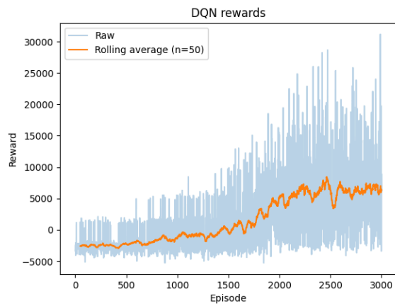
Figure 26: Neutral Agent v.s. Hybrid Opponent v2 (NEHY2)
