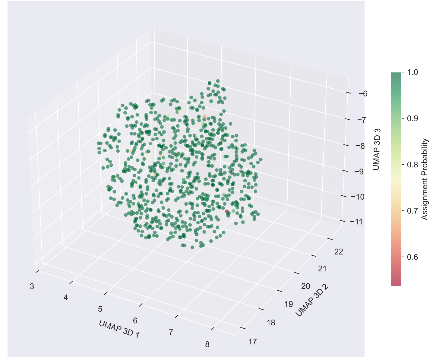
UMAP — Assignment Confidence
