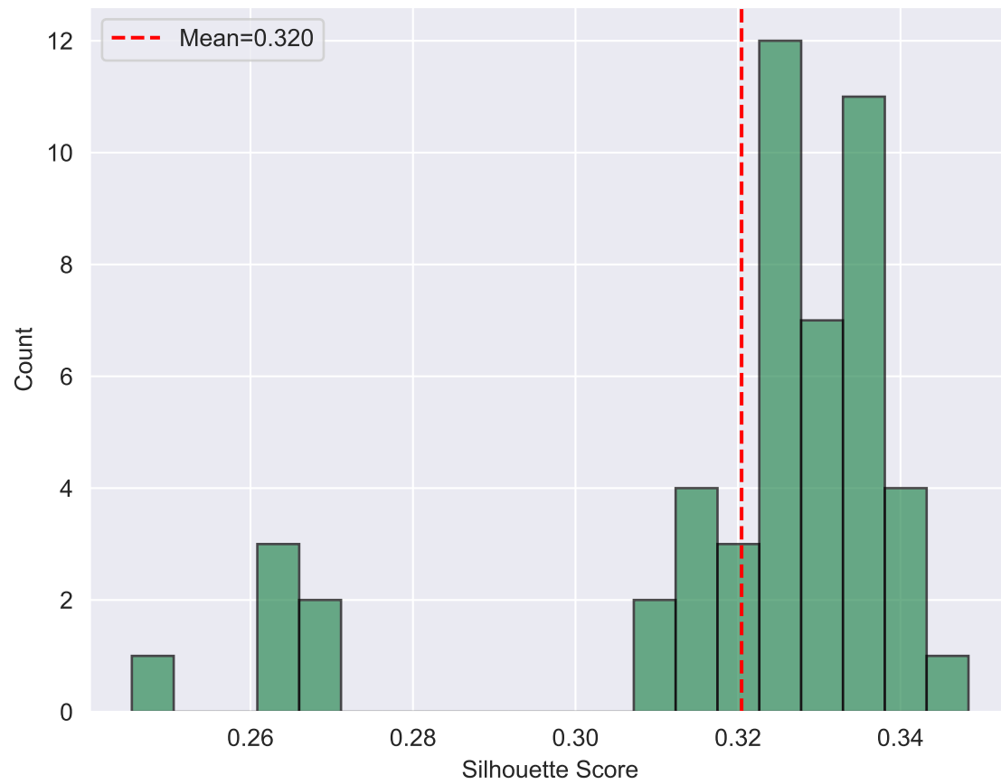
Silhouette Across Runs
