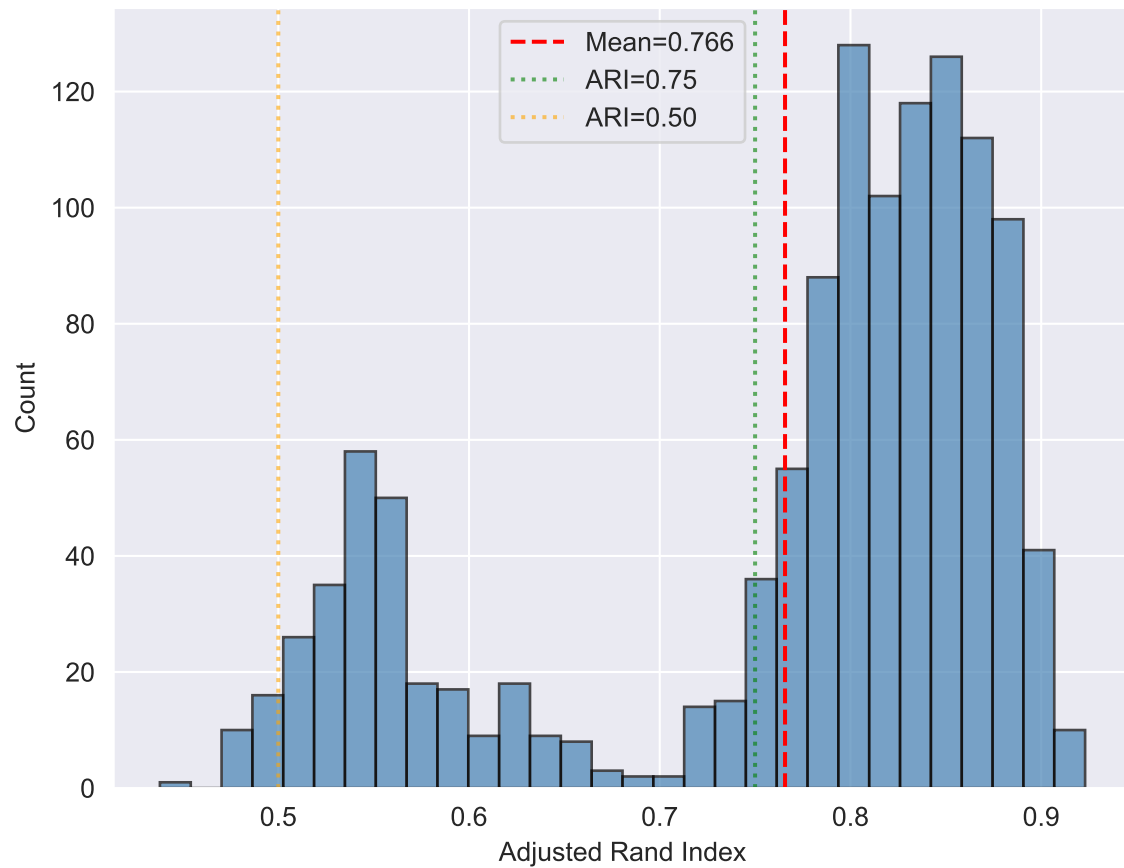
Pairwise ARI Across Runs (n_pairs=1225)
