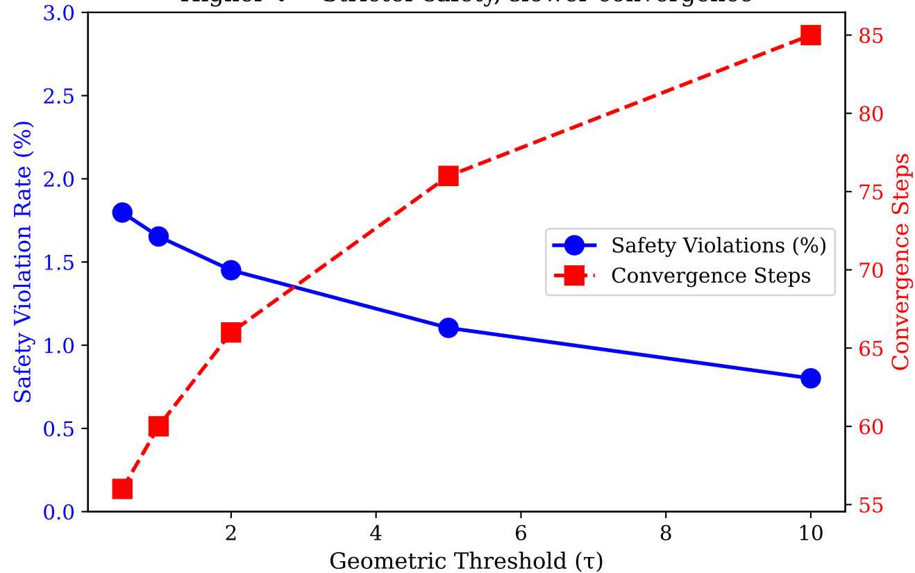
Effect of Geometric Threshold Higher \tau = Stricter safety, slower convergence
