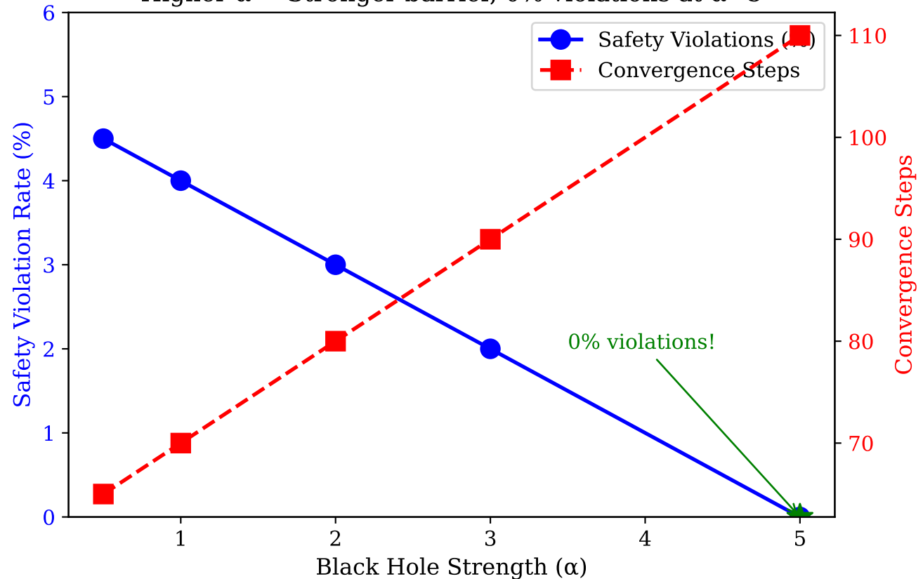
Effect of Black Hole Strength Higher \alpha = Stronger barrier, 0% violations at \alpha=5
