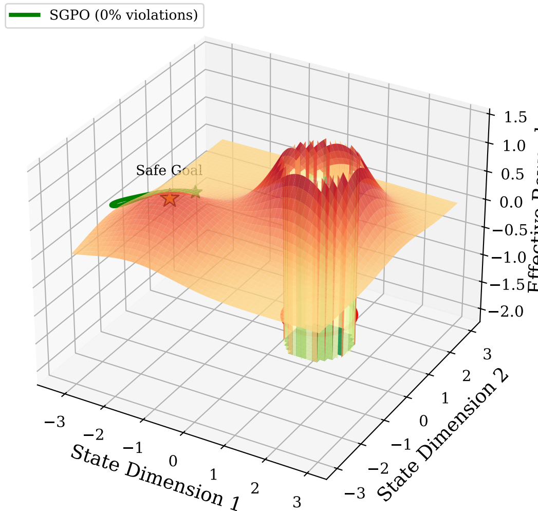
SGPO View: Geometric Singularity at Trap (Infinite cost = impassable barrier)
