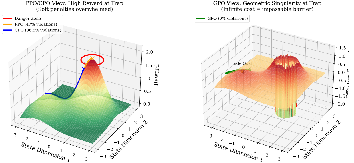
Figure 1. Reward Manifold Comparison. Left: PPO and CPO see the trap (red ring) as a region of high reward, causing them to spiral into it despite soft penalties. Right: GPO views the trap as a geometric singularity with infinite cost ( g(x) \rightarrow \infty ), creating an impassable barrier.
