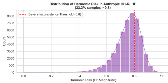
Figure 4. Harmonic risk in Anthropic HH-RLHF. Left: Histogram showing concentration around 0.75–0.80. Right: 33% of pairs exceed severe inconsistency threshold ( r \geq 0.8 ).
