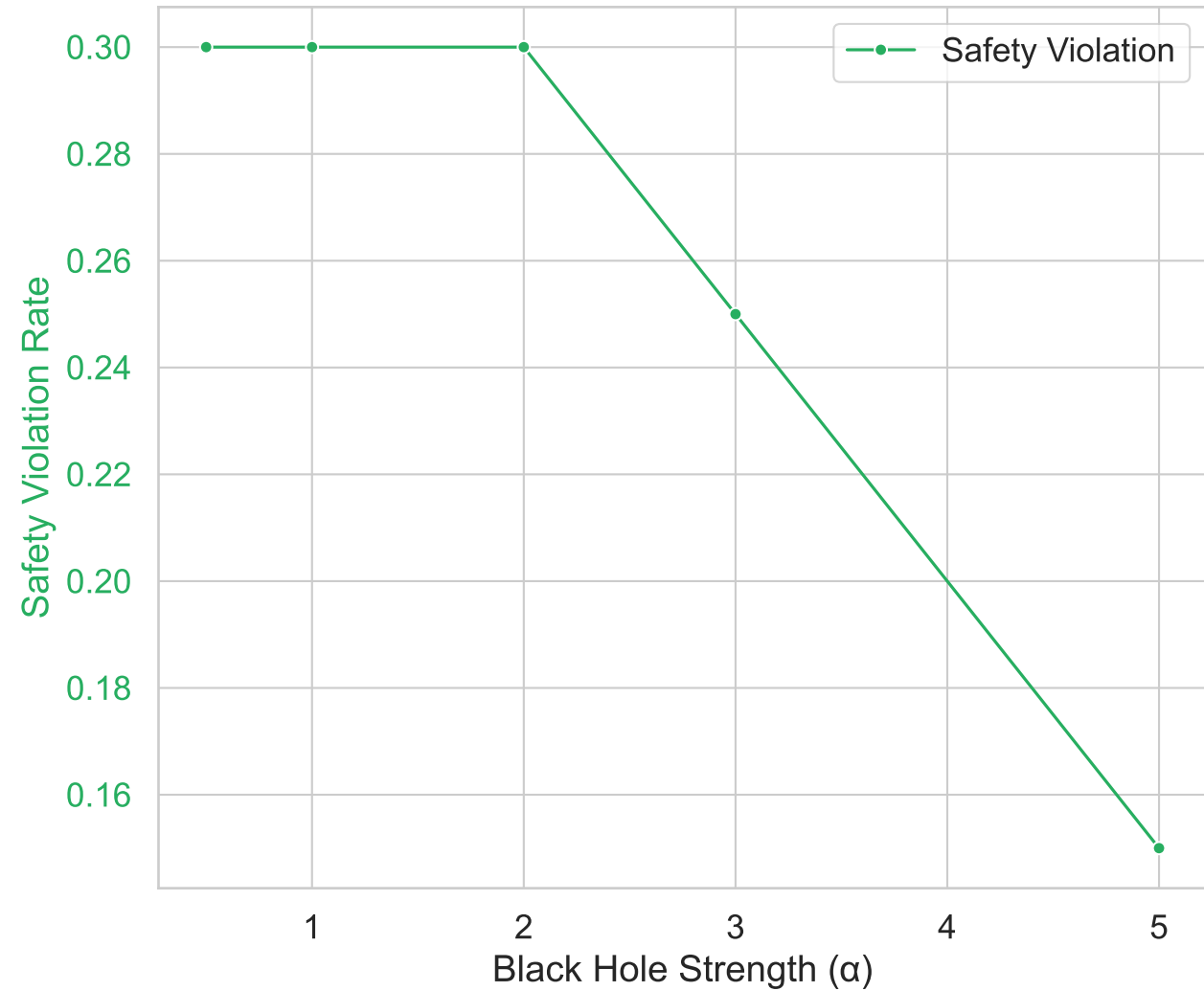
Effect of Black Hole Strength ( \alpha )
