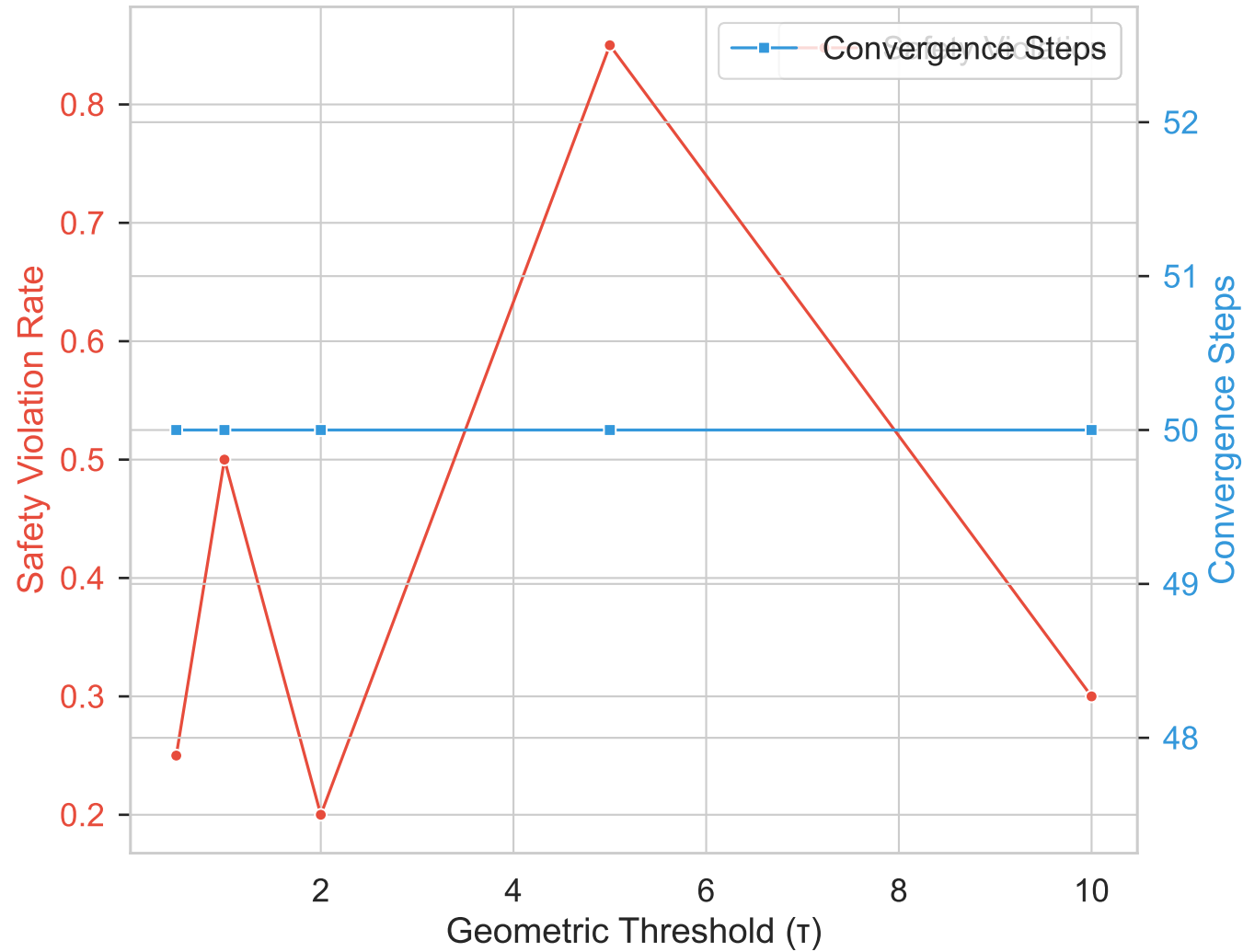
Effect of Geometric Threshold ( \tau )
