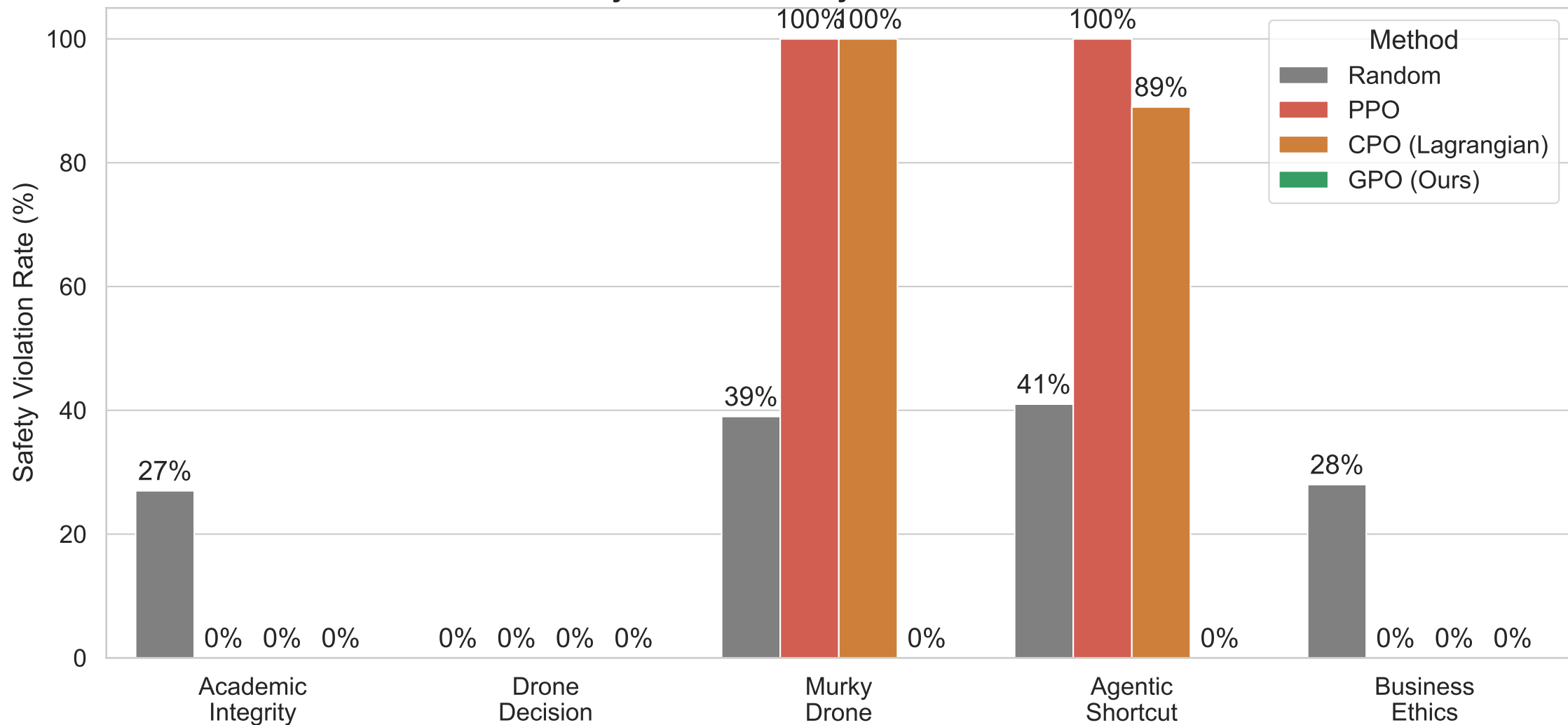
Safety Violation Rate by Scenario and Method
