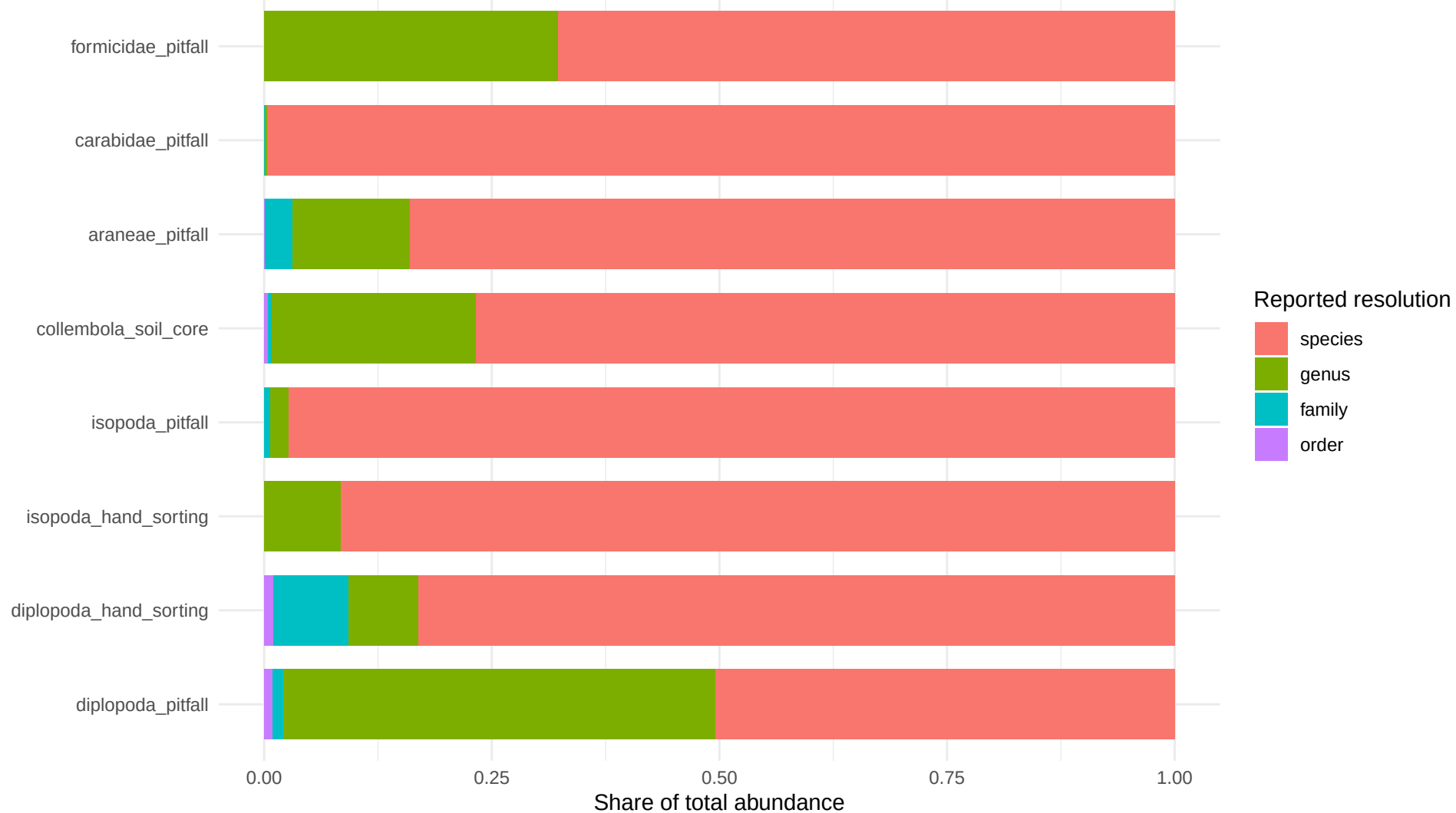
Taxonomic-resolution audit across RMQS 2024 assemblage × protocol datasets
