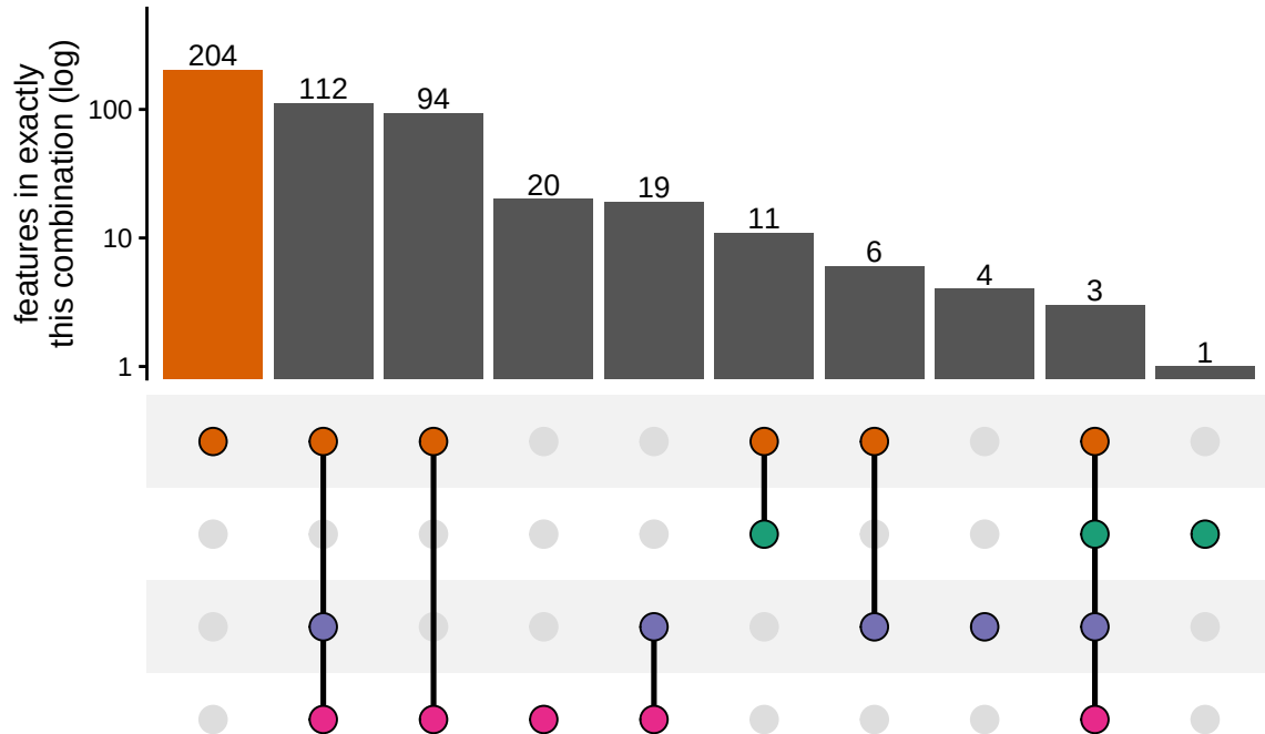
Feature membership across variate groups, patient=SARCO361_T1 (orange = treatment only)
