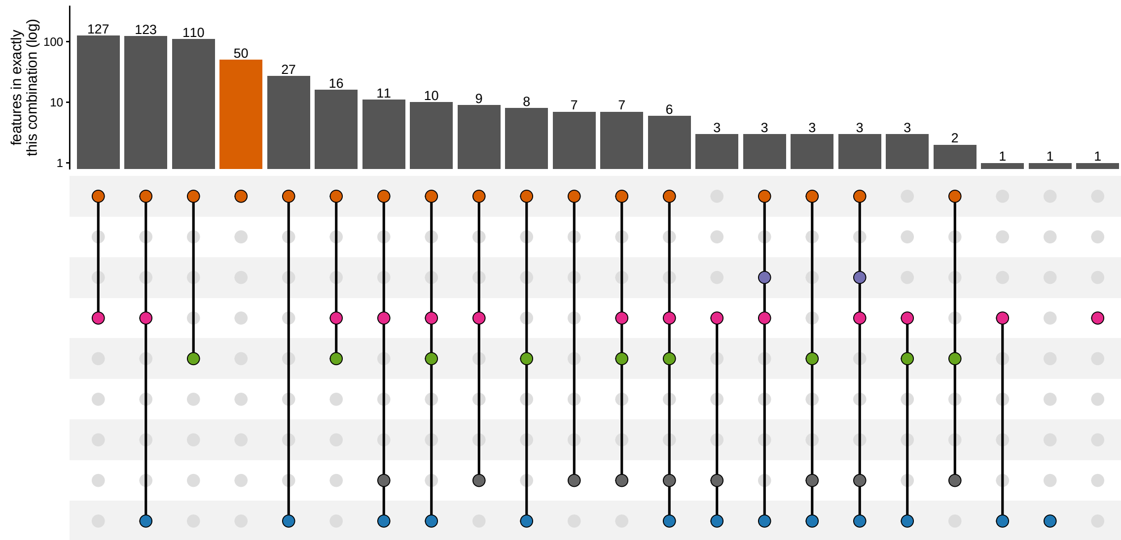
Feature membership across variate groups, patient=SARCO219_T2 (orange = treatment only)
