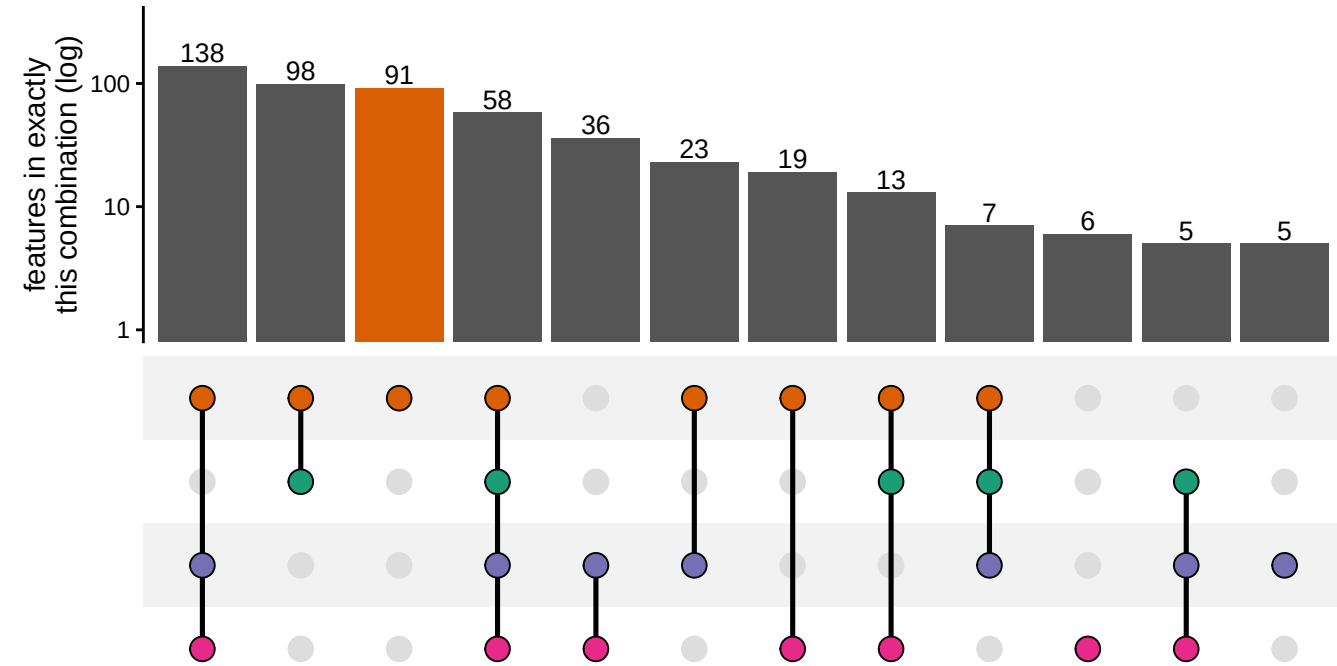
Feature membership across variate groups, patient=NF0016_T1 (orange = treatment only)
