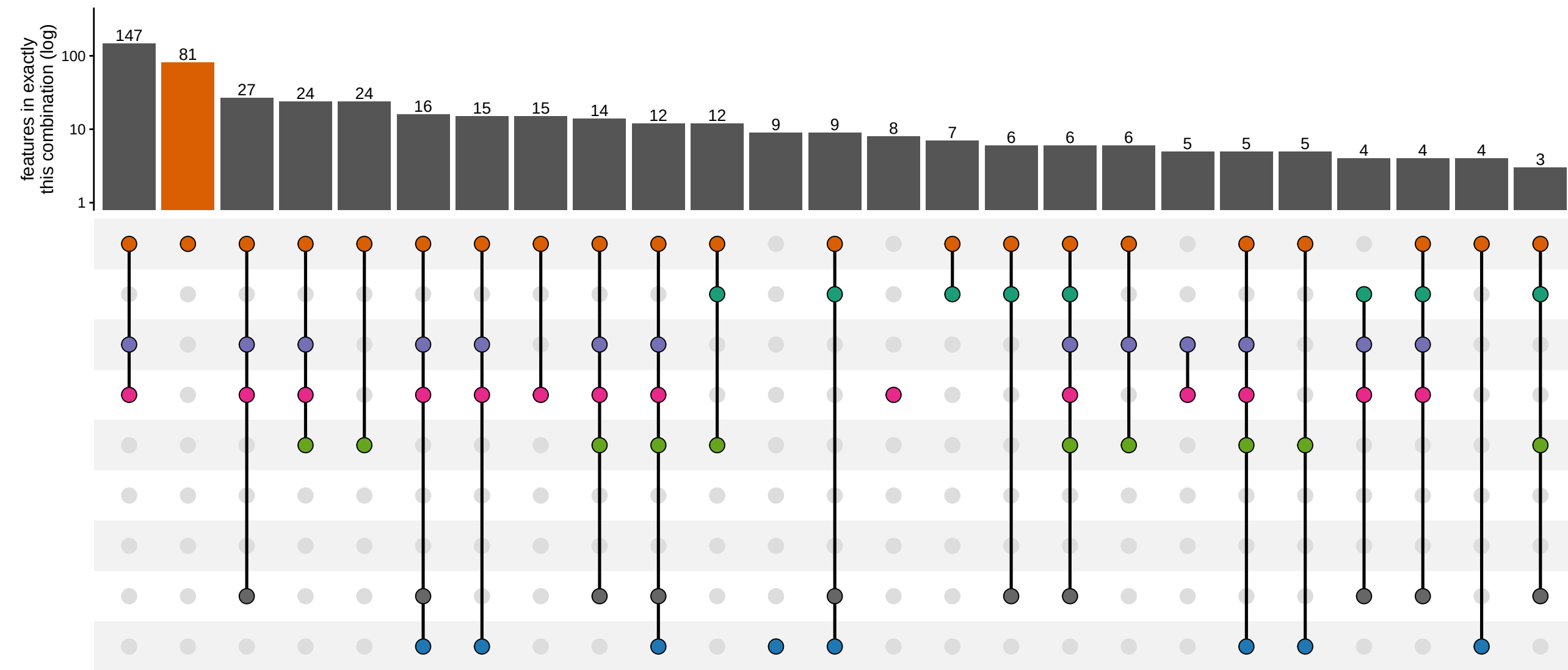
Feature membership across variate groups, patient=NF0014_T2 (top 25 of 49 combinations; orange = treatment only)
