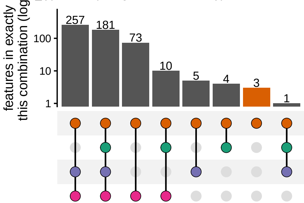
Feature membership across variate groups, tumor_type=cNF (orange = treatment only)
