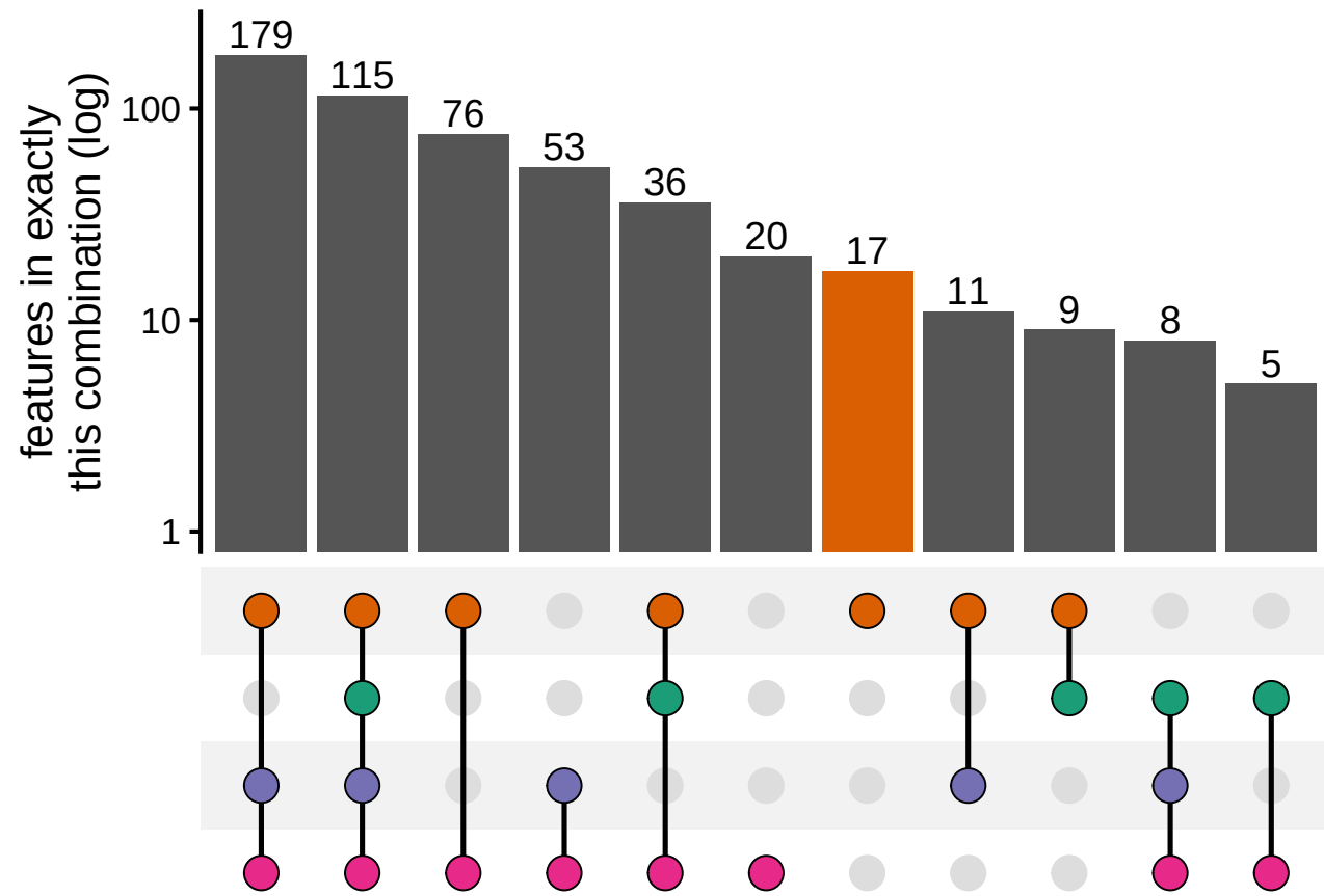
Feature membership across variate groups, treatment=Fimepinostat_1uM (orange = treatment only)
