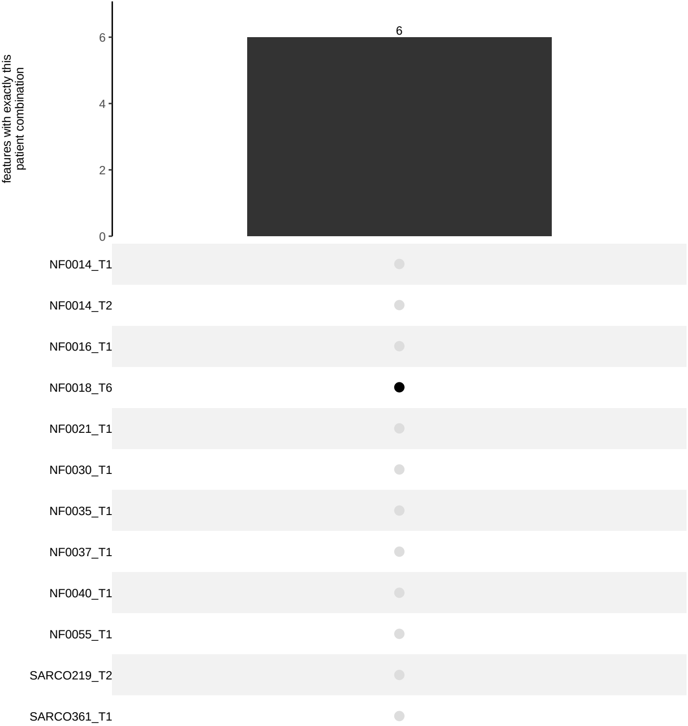
cell_count + manhattan_distance_from_center + cell_x_position | Mirdametinib_10uM Features significant for exactly these variates, by the patients they occur in (bars: number of features shared by exactly that patient combination)
