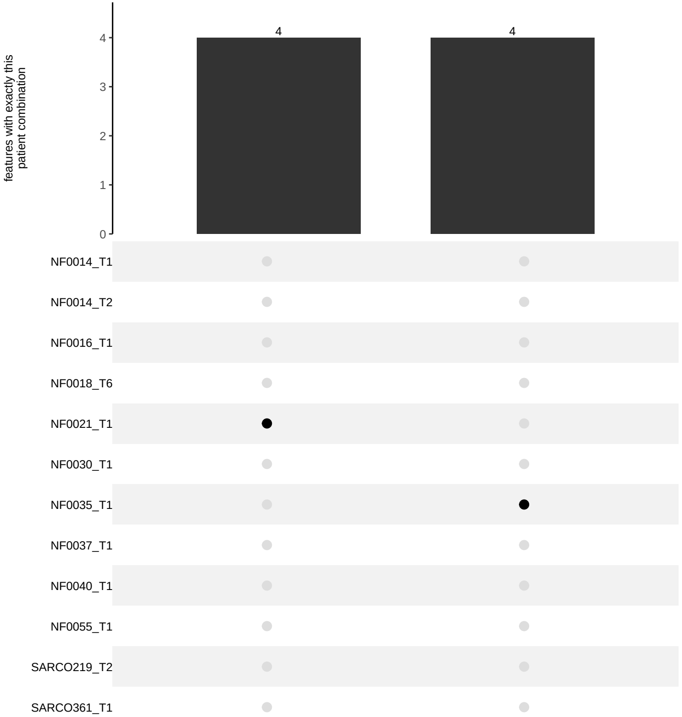
cell_count + manhattan_distance_from_center + cell_z_depth | Staurosporine_10nM Features significant for exactly these variates, by the patients they occur in (bars: number of features shared by exactly that patient combination)
