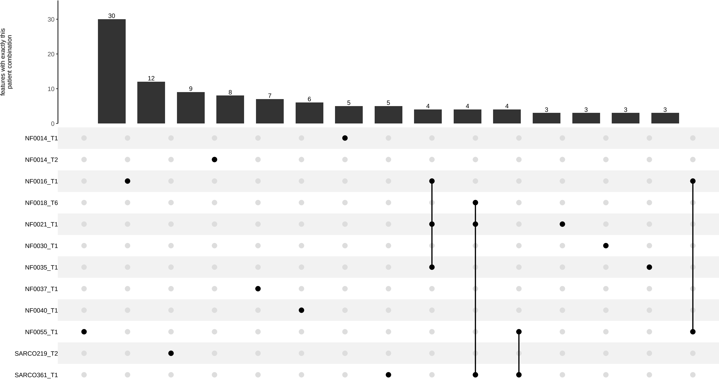
cell_z_position | Binimetinib_1uM Features significant for exactly these variates, by the patients they occur in (bars: number of features shared by exactly that patient combination)
