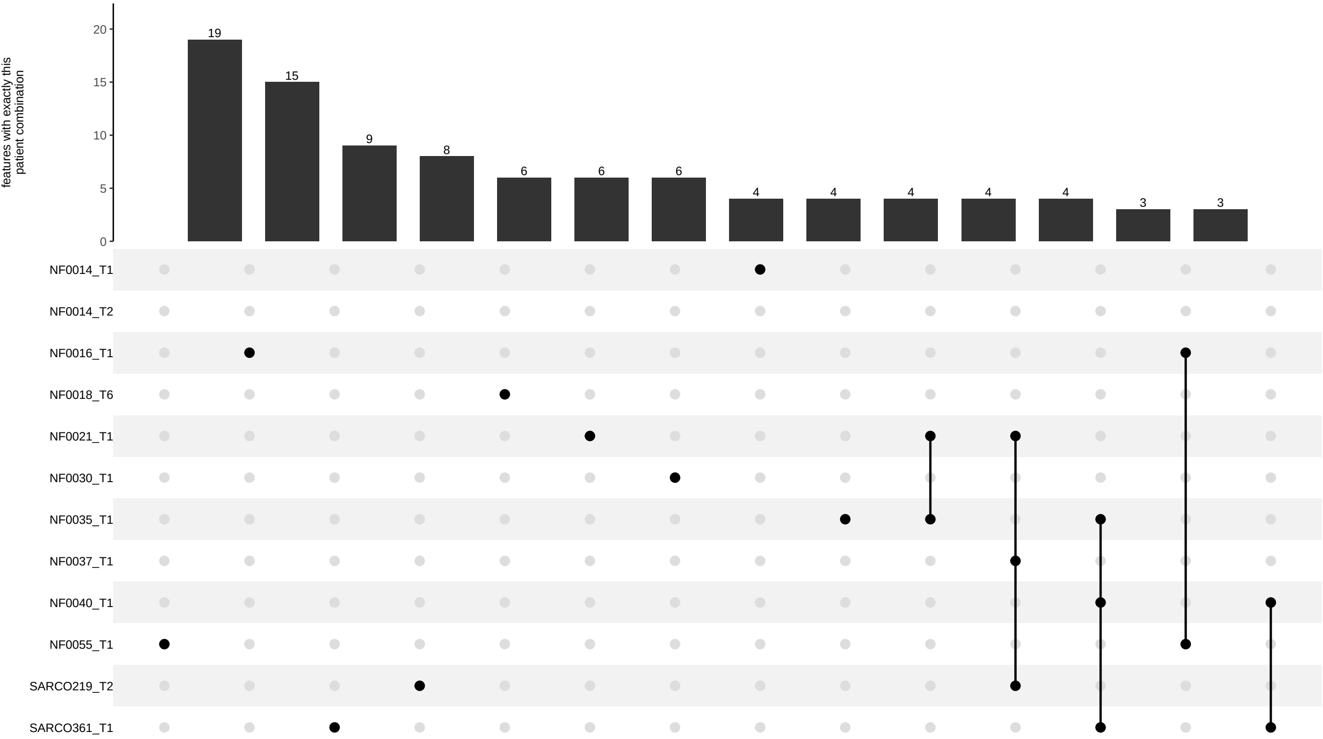
cell_z_position | Onalespib_1uM Features significant for exactly these variates, by the patients they occur in (bars: number of features shared by exactly that patient combination)
