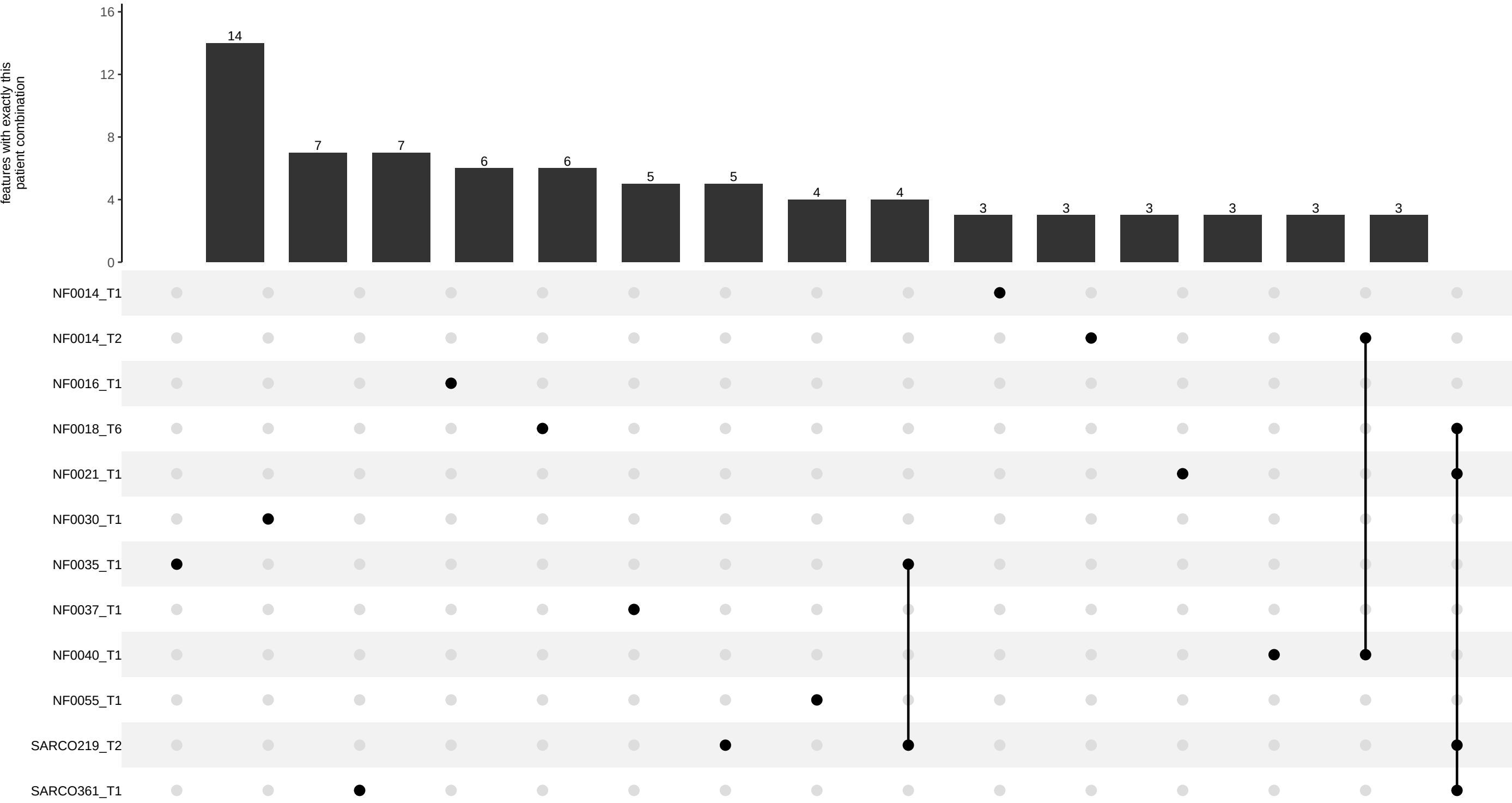
cell_z_position | Imatinib_1uM Features significant for exactly these variates, by the patients they occur in (bars: number of features shared by exactly that patient combination)
