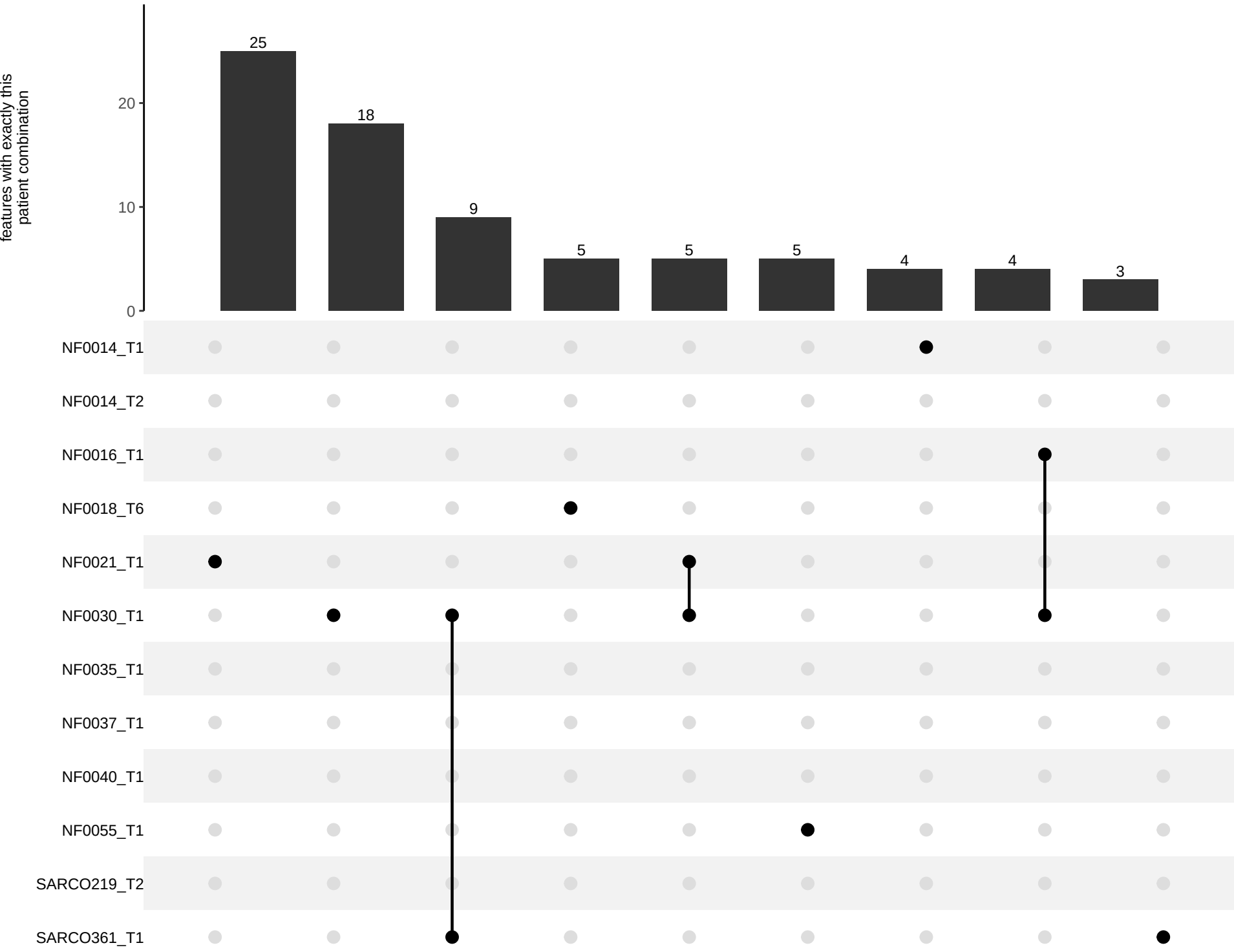
cell_z_position + cell_z_depth | Onalespib_1uM Features significant for exactly these variates, by the patients they occur in (bars: number of features shared by exactly that patient combination)
