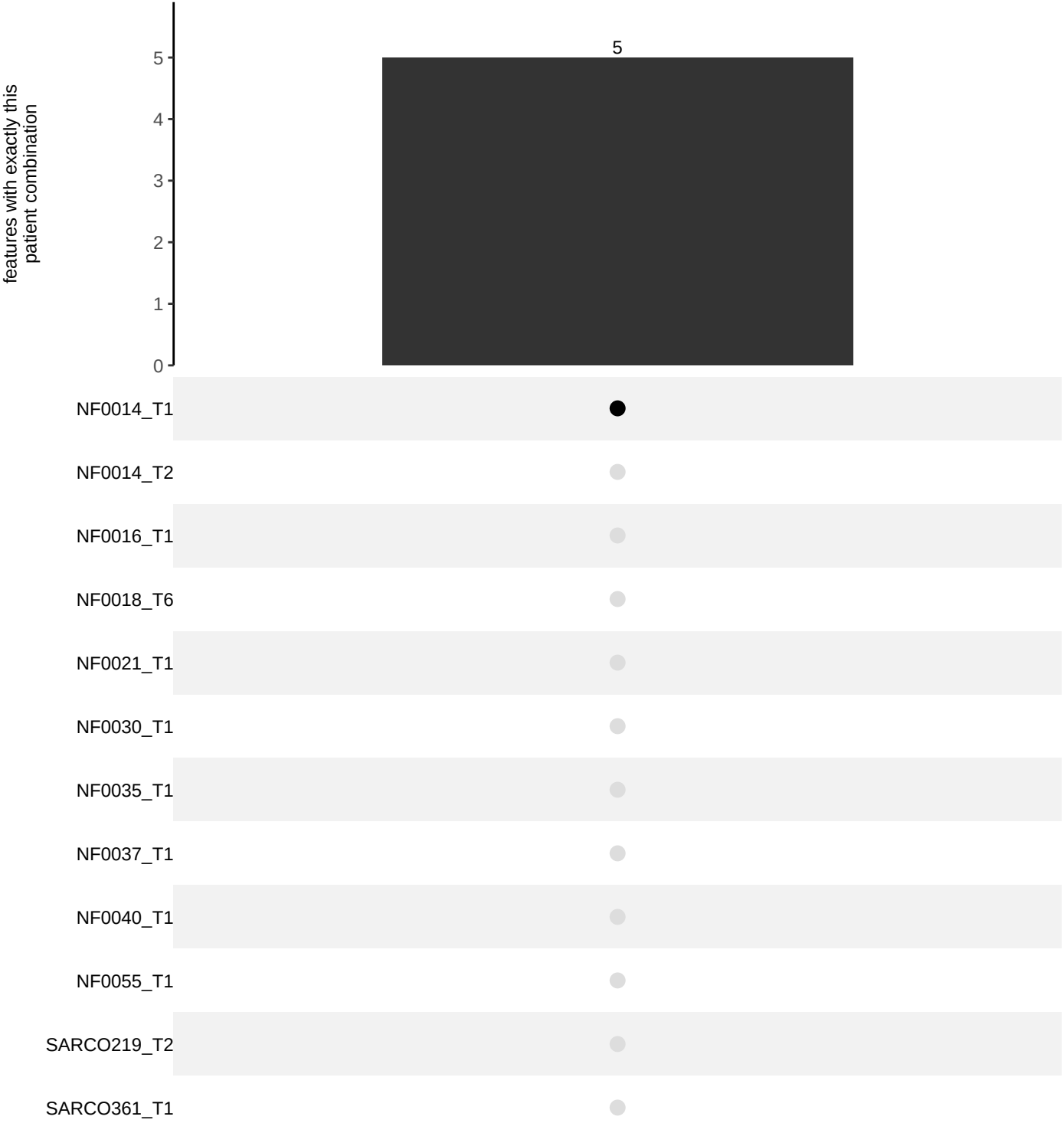
organoid_count + manhattan_distance_from_center + cell_z_position | Linsitinib_1uM Features significant for exactly these variates, by the patients they occur in (bars: number of features shared by exactly that patient combination)
