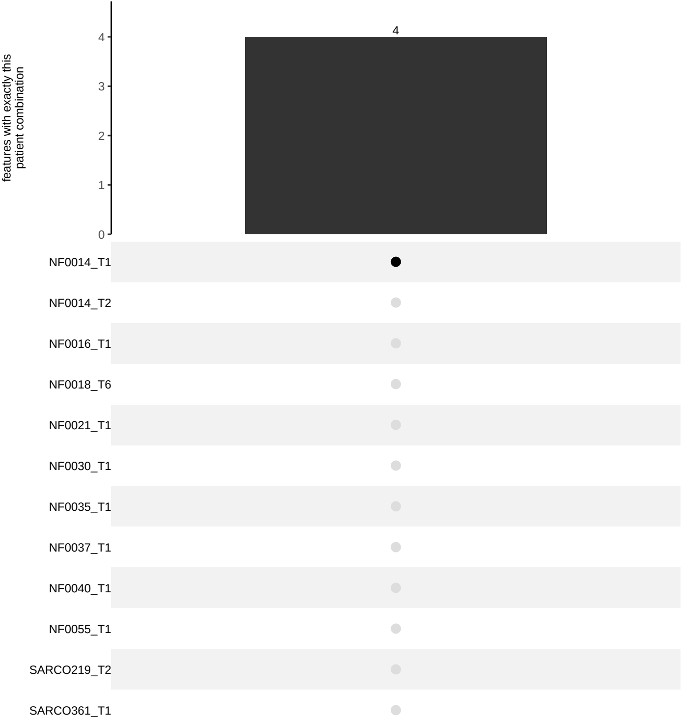
treatment + cell_per_organoid_count + cell_y_position + cell_z_depth | Onalespib_1uM Features significant for exactly these variates, by the patients they occur in (bars: number of features shared by exactly that patient combination)
