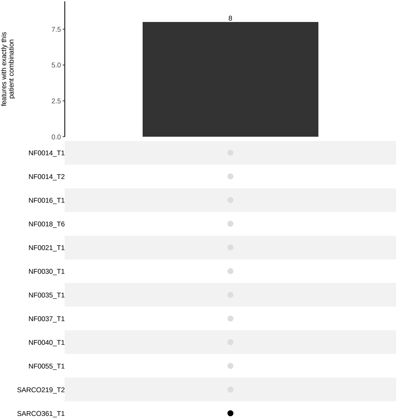
treatment + cell_per_organoid_count + cell_z_position + cell_z_depth | Linsitinib_1uM Features significant for exactly these variates, by the patients they occur in (bars: number of features shared by exactly that patient combination)
