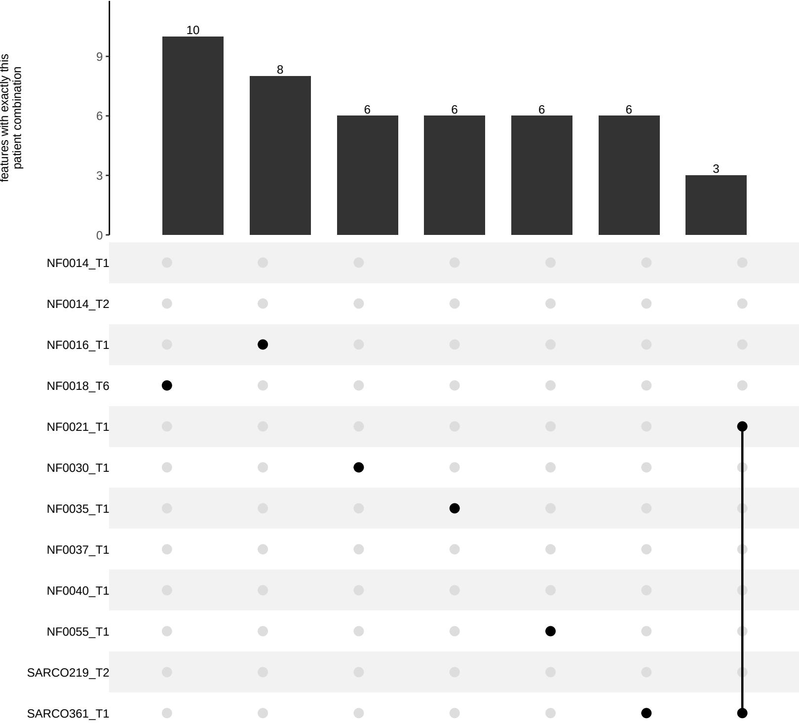
treatment + cell_y_position | Digoxin_1uM Features significant for exactly these variates, by the patients they occur in (bars: number of features shared by exactly that patient combination)
