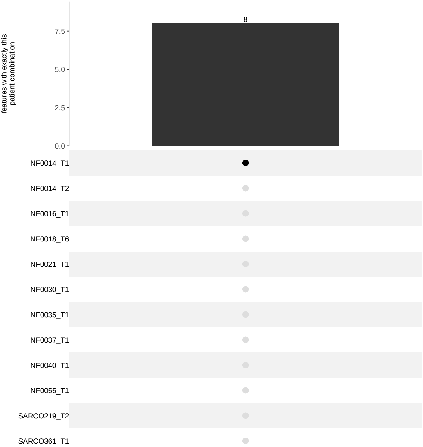
treatment + organoid_count + cell_per_organoid_count + cell_z_depth | Digoxin_1uM Features significant for exactly these variates, by the patients they occur in (bars: number of features shared by exactly that patient combination)
