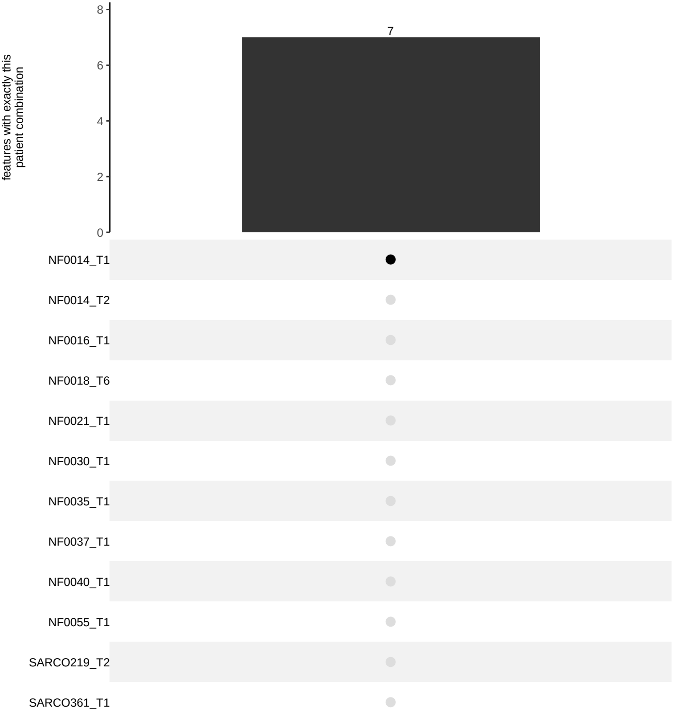
treatment + organoid_count + cell_per_organoid_count + cell_z_depth | Copanlisib_1uM Features significant for exactly these variates, by the patients they occur in (bars: number of features shared by exactly that patient combination)
