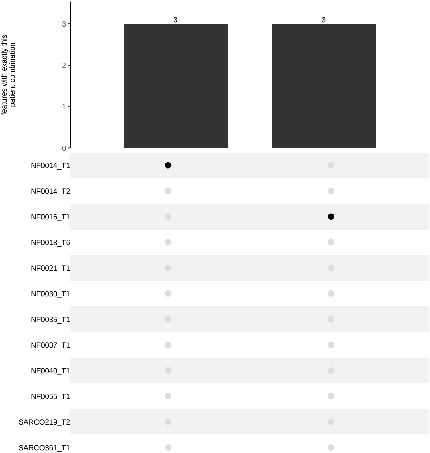
treatment + organoid_count + cell_per_organoid_count + cell_z_depth | Linsitinib_1uM Features significant for exactly these variates, by the patients they occur in (bars: number of features shared by exactly that patient combination)
