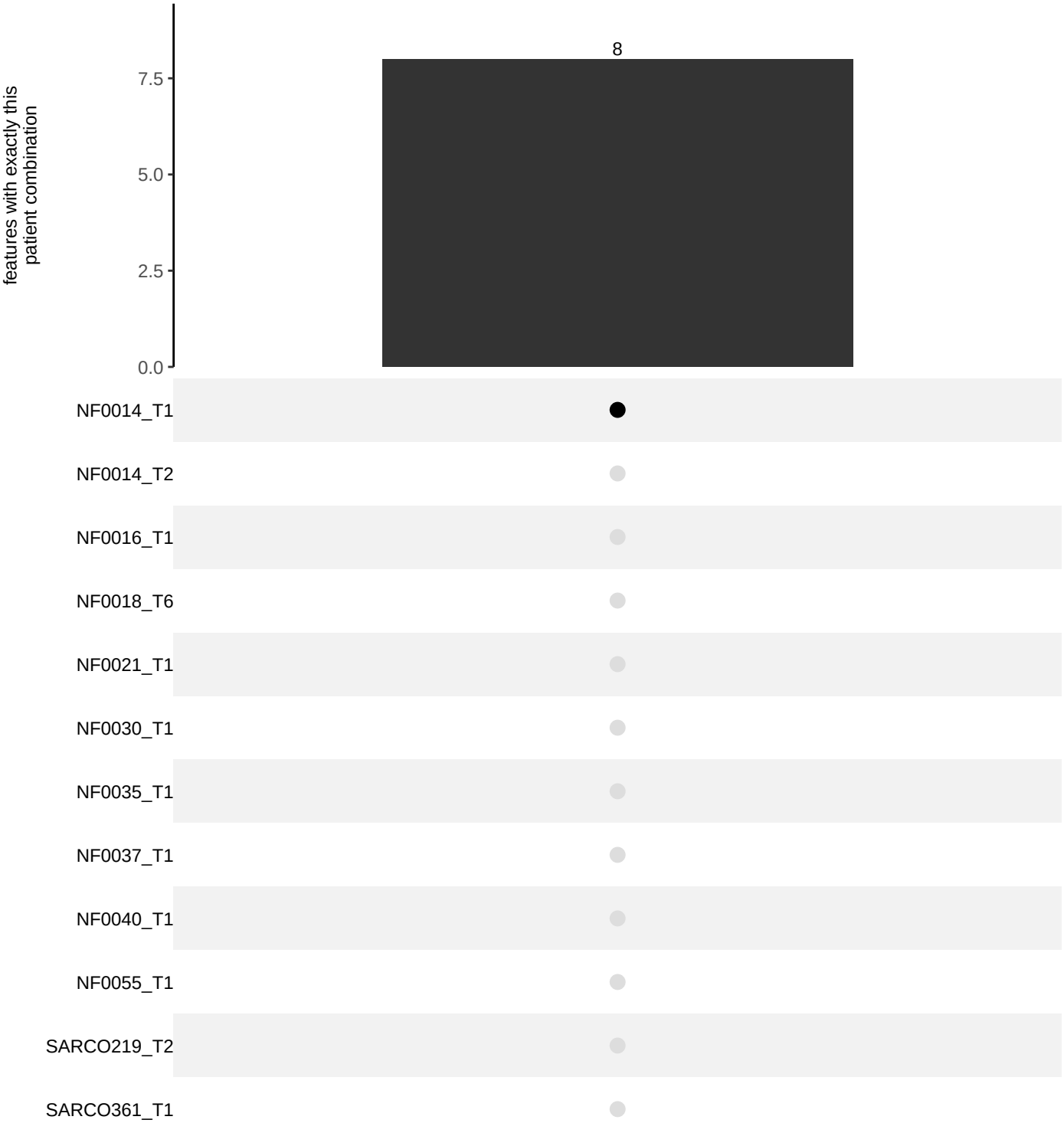
treatment + organoid_count + cell_per_organoid_count + cell_z_depth | Onalespib_1uM Features significant for exactly these variates, by the patients they occur in (bars: number of features shared by exactly that patient combination)
