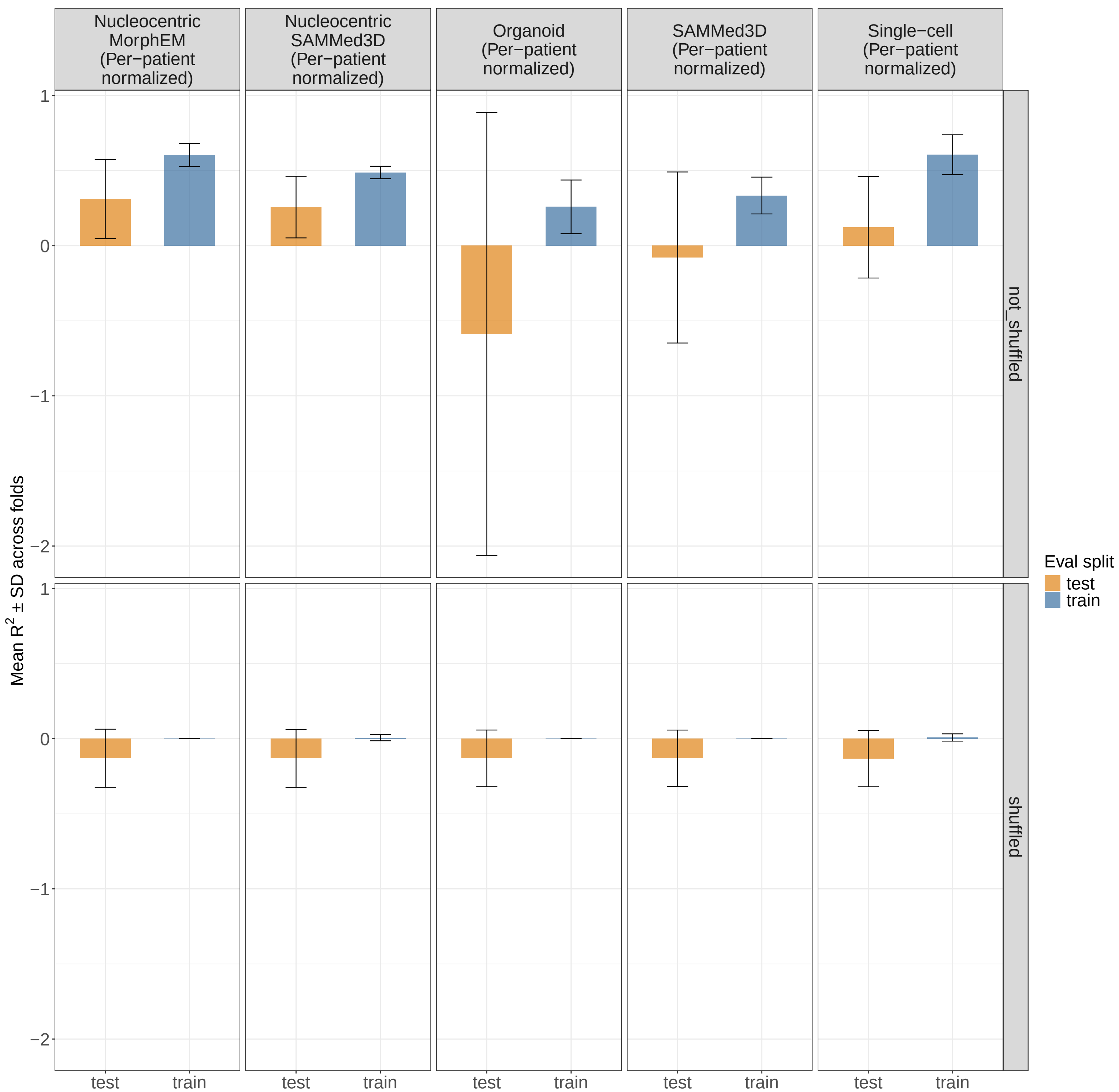
Model performance ( R^2 ) by profile and feature type ... lopo
