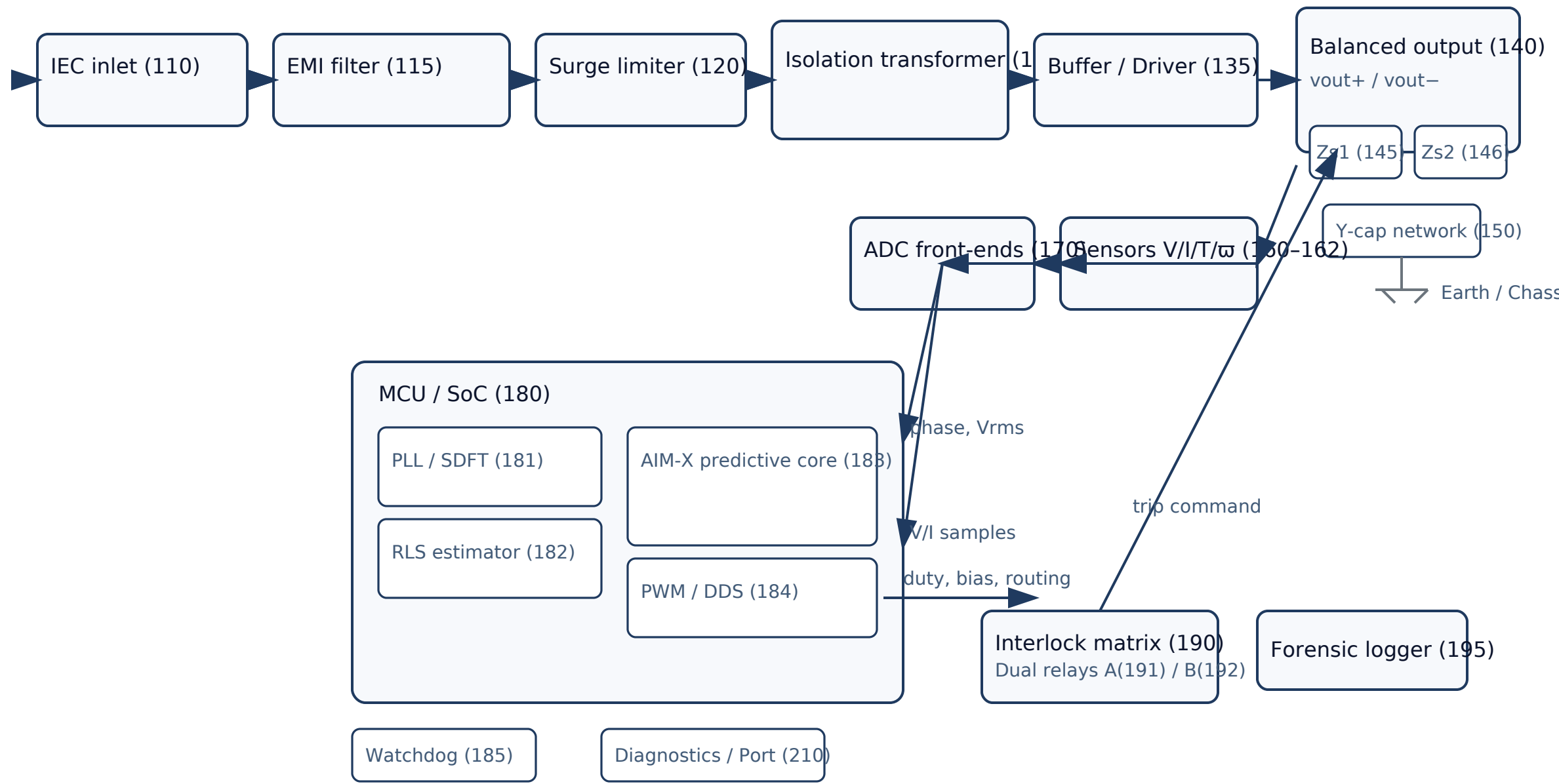
FIG. 1 — System Overview and Functional Block Diagram
