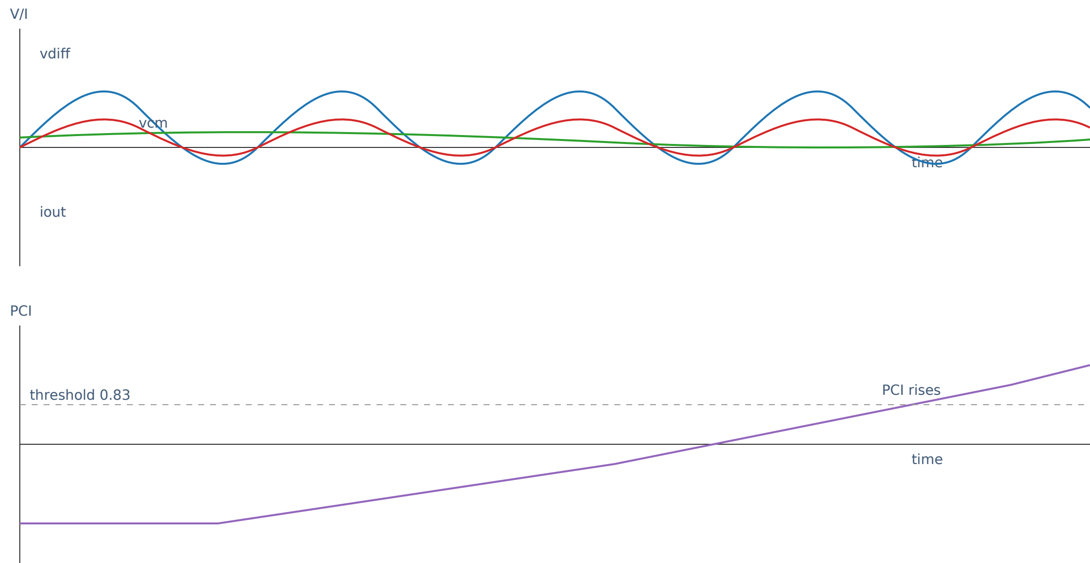
FIG. 4 — Waveforms: vdiff, vcm, iout, PCI
