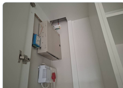
Plate 045 Alarm and security installation in the service cupboard
