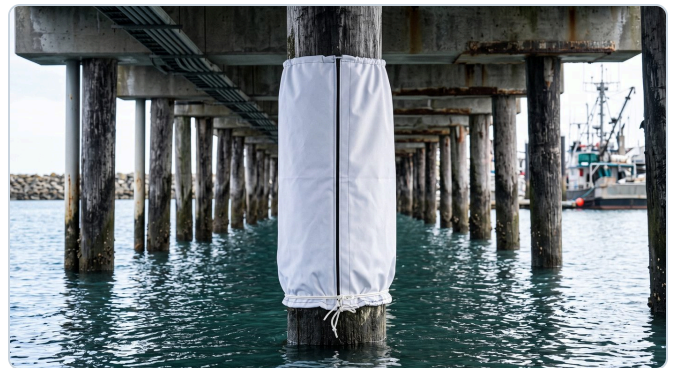
Installed at the waterline, drawstring cinched to the pile (illustrative rendering)
