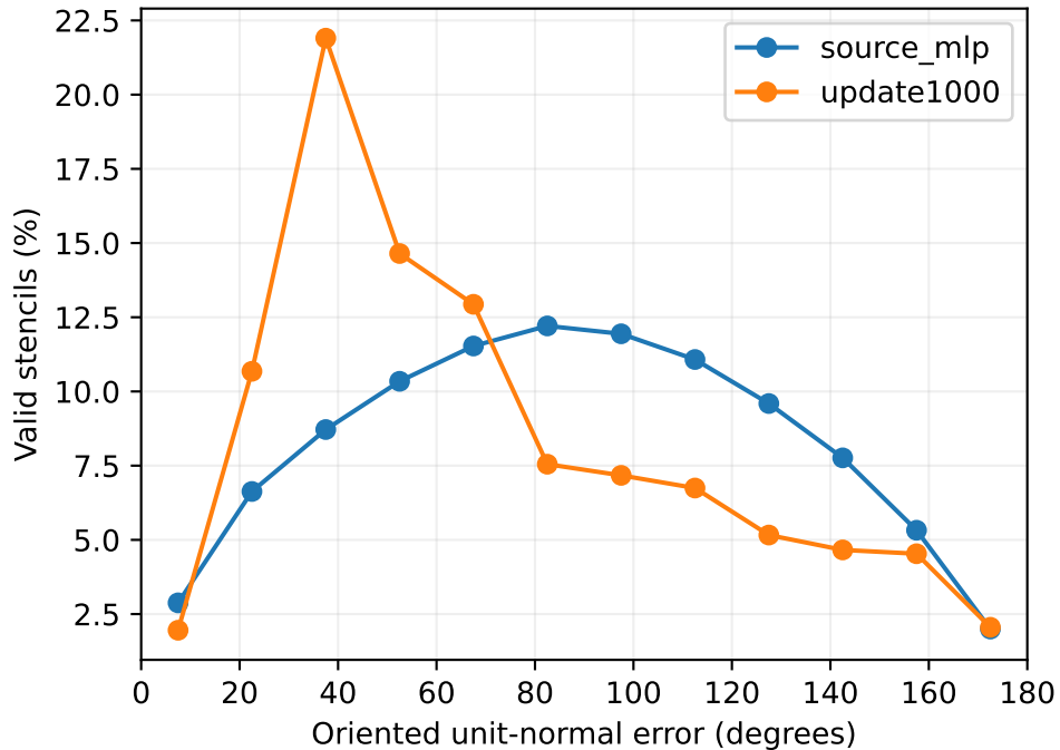
Heavy occlusion / proxy
