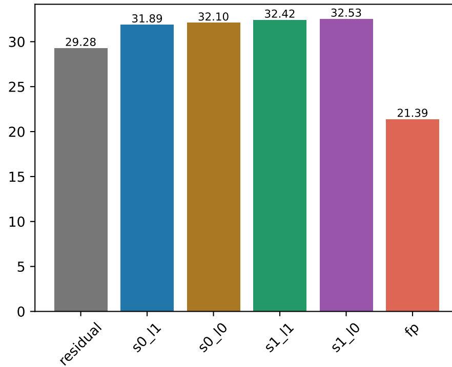
Visibility &lt; 0.3: strict ADD-S (%)
