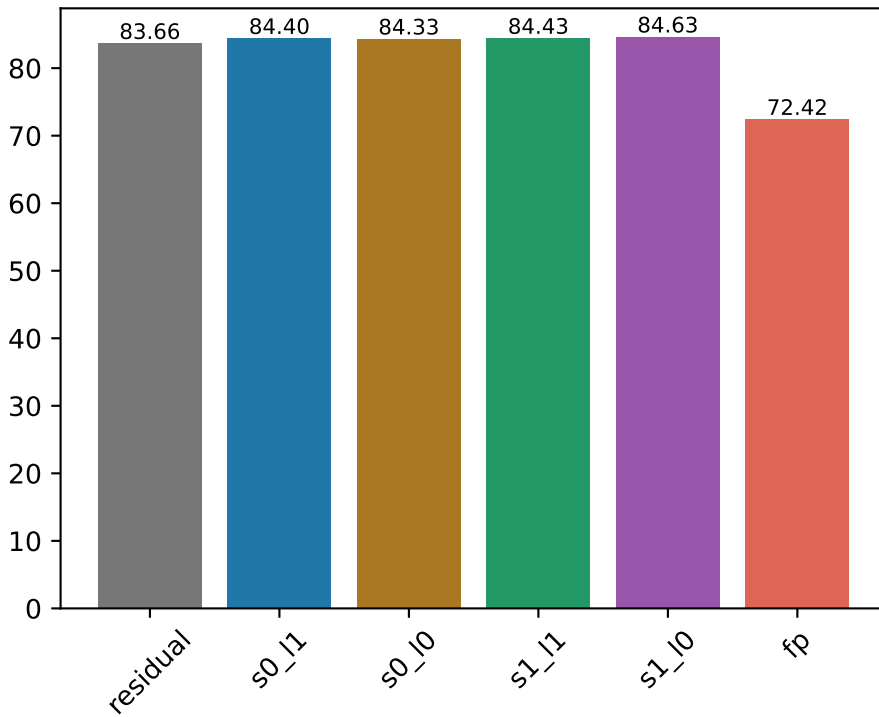
All: strict ADD-S (%)
