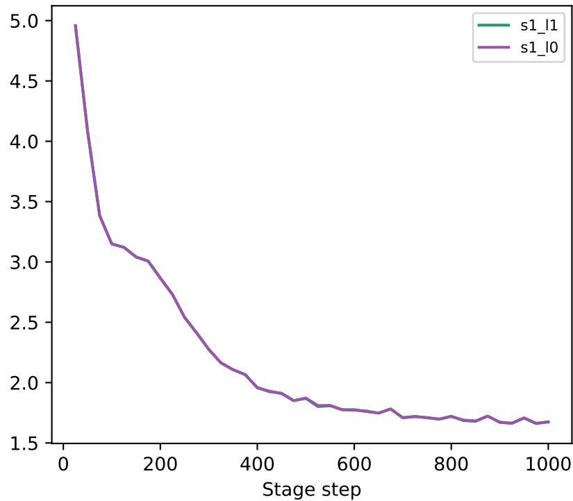
Spatial CE (training support)
