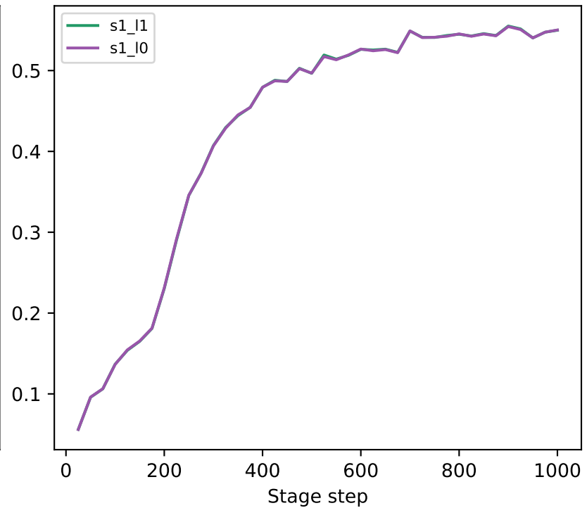
Attention target hit rate (training support)
