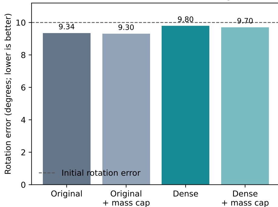
Pose: no consistent downstream gain
