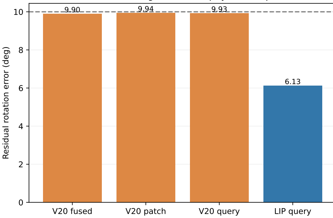
Frozen-feature ridge: held-out physical sequences
