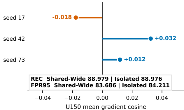
b Strong e5: effective sharing
