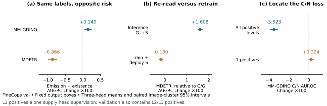
Figure 1. From an endpoint difference to an explanation to investigate. All panels use FineCops validation with fixed Native output boxes. (a) Changing existence labels to correct-emission labels raises complete risk on MM-GDINO and lowers it on MDETR. (b) For MDETR emission confidence, reading the selected query only at inference raises risk, whereas training and deploying that readout lowers it; both reference the G-trained/G-deployed head. (c) MM-GDINO’s correct-output/no-target ( C/N ) target effect changes sign within L1, the only positive difficulty level supplying head-loss supervision. Panels (a,b) show AUGRC differences, where lower is better; (c) shows AUROC differences, where positive means a larger pairwise AUROC. Intervals resample images for the fixed three-head mean. The L1 comparison is not a training-coverage intervention.
