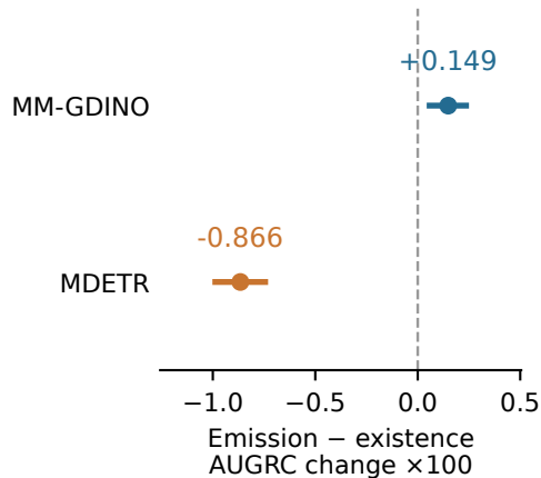
(a) Same labels, opposite risk
