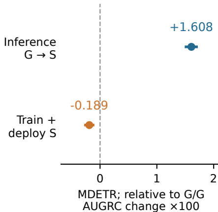
(b) Re-read versus retrain
