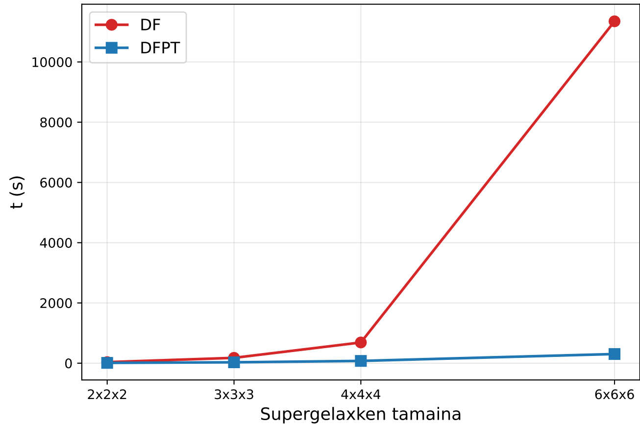
DFPT vs DF
