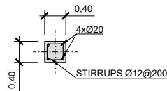
SECTION B-B SCALE 1:50
