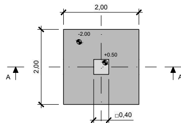
TYPE 01 PLAN VIEW SCALE 1:50
