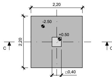
TYPE 02 PLAN VIEW SCALE 1:50
