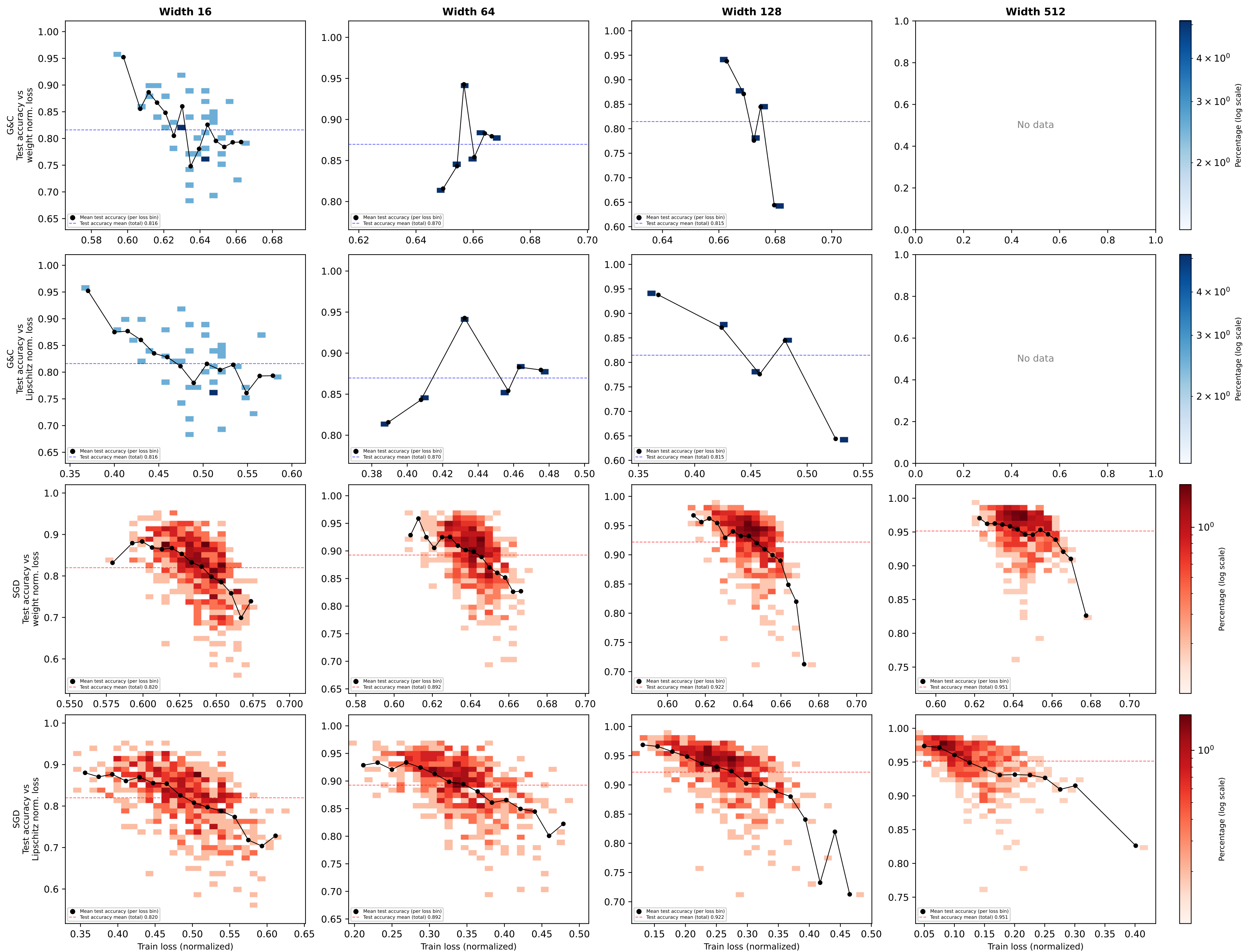
Test Accuracy vs. Normalised Train Loss — Kink dataset Width sweep — Init: U[-1, 1]
